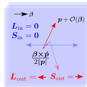
FIG. 1 (color online). Side jump.
