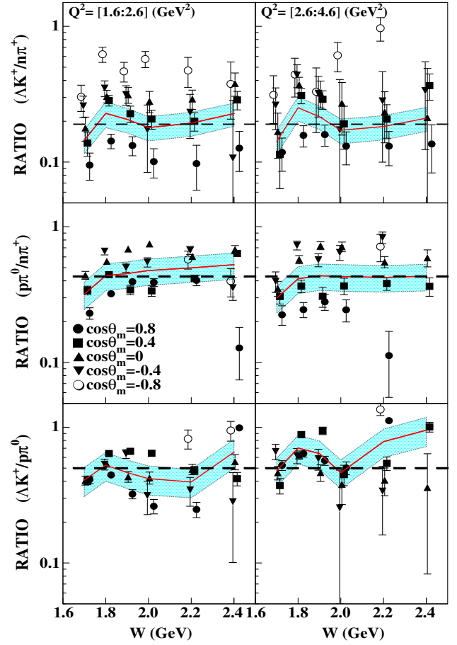
FIG. 2 (color online). Ratio of the three exclusive cross sections, displayed as in Fig. 1, but plotted versus W with different bins of \cos\theta_m^* shown as different symbols.
