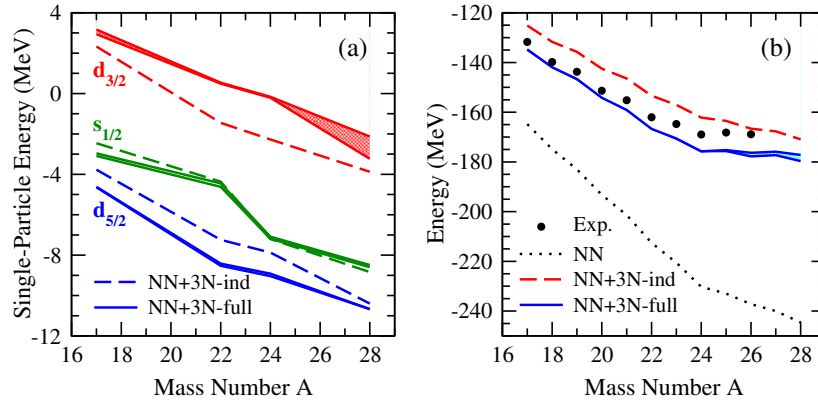
FIG. 1 (color online). Single-particle energy evolution (a) and ground-state energies (b) for the indicated A -dependent Hamiltonians with \lambda_{\text{SRG}} = 1.88 \text{ fm}^{-1} . The range of NN + 3N-full ( \Lambda_{3\text{N}} = 400 \text{ MeV} ) results for \hbar\omega = 20, 24 \text{ MeV} is given by the shaded bands.
