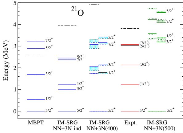
FIG. 2 (color online). Excited-state spectrum of ^{21}\text{O} for IM-SRG Hamiltonians based on NN + 3N-induced and NN + 3N-full Hamiltonians for \Lambda_{3\text{N}} = 400, 500 MeV, with \hbar\omega = 20 MeV (dotted) and \hbar\omega = 24 MeV (solid), compared with MBPT (NN + 3N) and experiment [48]. NN + 3N-full results are given in two columns: \lambda_{\text{SRG}} = 1.88 \text{ fm}^{-1} (left) and \lambda_{\text{SRG}} = 2.24 \text{ fm}^{-1} (right). The neutron-separation threshold is given by black dot-dashed lines.
