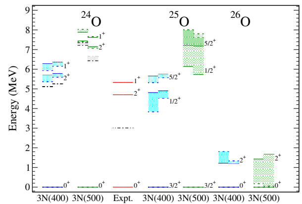
FIG. 5 (color online). Excited state spectra of ^{24-26}\text{O} for \Lambda_{3\text{N}} = 400, 500 MeV NN + 3N-full Hamiltonians with \hbar\omega = 20 MeV (dotted), \hbar\omega = 24 MeV (solid), and \lambda_{\text{SRG}} dependence as in Fig. 2, compared to experiment for ^{24}\text{O} [52,53].
