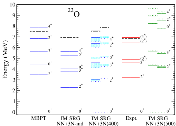
FIG. 3 (color online). Excited state spectrum for ^{22}\text{O} as in Fig. 2, with experimental values from Refs. [48,49].
