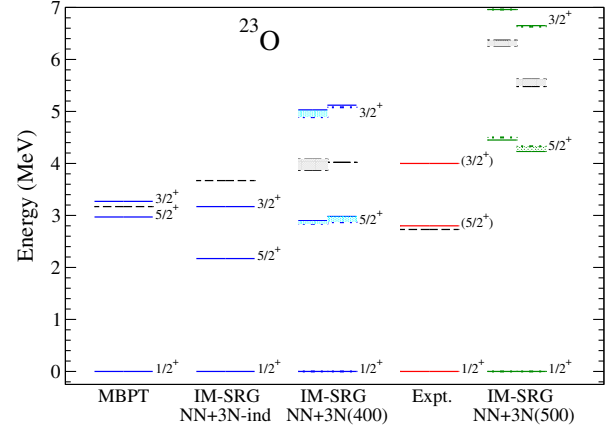
FIG. 4 (color online). Excited state spectrum of ^{23}\text{O} as in Fig. 2, with experimental values from Refs. [50,51].
