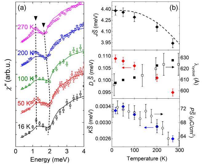
FIG. 4 (color online). (a) Temperature dependence of \text{Im}[\chi(\mathbf{q}, \omega)] at \mathbf{q} = (1, 0, -1) with best fit curves. (b) Temperature dependence of J\tilde{S} , D_u\tilde{S} , K\tilde{S} , and a period of the magnetic cycloid with the arrows representing typical error bars. We estimated the temperature dependence of the moment \tilde{S} (dashed line) and the electric polarization ( P ) using the structural data taken from Ref. [20] while the open symbol of \lambda is taken from Ref. [19].
