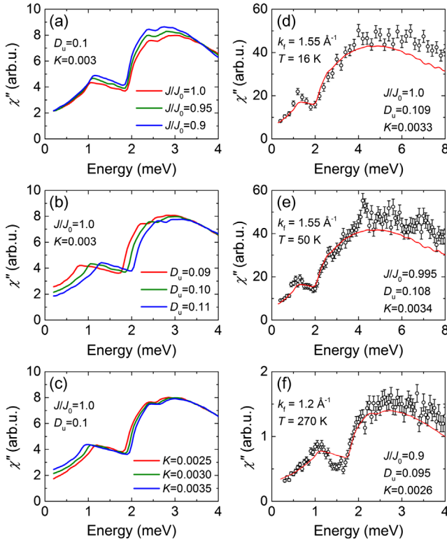
FIG. 3 (color online). Simulation results for different (a) J/J_0 , (b) D_u , and (c) K . Best fit results with k_f = 1.55 \text{ \AA}^{-1} at (d) 16 K, (e) 50 K, and (f) with k_f = 1.2 \text{ \AA}^{-1} at 270 K.
