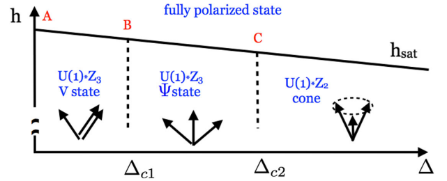
FIG. 2 (color online). The phase diagram of the XXZ model in a magnetic field near a saturation value, \Delta = (J - J_z)/J . The cone and V states are the same as in Fig. 1, but the transformation from one phase to the other with increasing spin exchange anisotropy proceeds differently from the case of spatial exchange anisotropy and involves one intermediate coplanar commensurate phase with a \Psi -like spin pattern.
