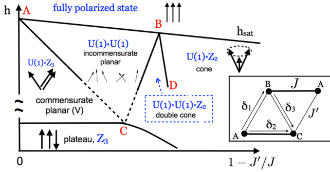
FIG. 1 (color online). Phase diagram of the spatially anisotropic triangular lattice antiferromagnet with large S near the saturation field, as a function of spatial anisotropy of the interactions. The phases at small and large anisotropy are the commensurate coplanar V phase, whose order parameter manifold is U(1) \times Z_3 , and incommensurate noncoplanar chiral phase, which lives in the U(1) \times Z_2 manifold. In between, there are two incommensurate phases: a coplanar phase, with U(1) \times U(1) symmetry, and a noncoplanar double cone phase, which is characterized by the U(1) \times U(1) \times Z_2 manifold. Line AC denotes the CI transition from the V phase to the incommensurate coplanar phase. The inset shows the geometry of the lattice: exchange is J on horizontal bonds (bold) and J' on diagonal bonds (thin).
