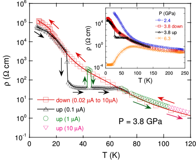
FIG. 2 (color online). Resistivity of a \text{GaTa}_4\text{Se}_8 single crystal (sample B) measured within the coexistence region as a function of temperature at 3.8 GPa. The commutation metal insulator in the heating process is controlled by a small bias current (see the text). Inset: Overall behavior of resistivity as a function of temperature for different pressures (2.4 GPa for sample A and 3.8 and 6 GPa for sample B).
