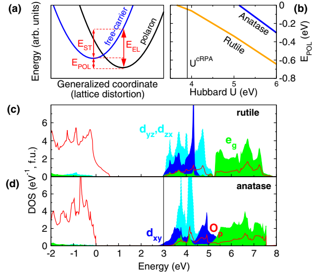
FIG. 1 (color online). Calculated polaronic stability for bulk TiO 2 rutile and anatase. (a) Configuration coordinate diagram showing the polaronic ( E_{POL} ), lattice ( E_{ST} ), and electronic ( E_{EL} ) energies as a function of lattice distortion for the polaronic and delocalized solution. (b) E_{POL} as a function of Hubbard U in bulk rutile (orange) and anatase (blue). The vertical line indicates the ab initio U^{cRPA} . Orbitally decomposed density of states (DOS) in rutile (c) and anatase (d), aligned with respect to the Ti core levels.
