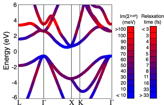
FIG. 2 (color online). The band structure of Si, together with a color map of the \text{Im}(\Sigma_{n,\mathbf{k}}^{e\text{-ph}}) and relaxation time.
