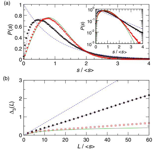
FIG. 3 (color online). (a) The distribution of the spacing between consecutive unfolded singular values obtained from a bipartition at the middle of a n = 16 qubit string at the end of the heating period ( M_h = 512 ). Solid black circles are for two-qubit gate heating and open red squares are for heating with a mixture of two-qubit and Toffoli gates. Solid green line: GOE prediction. Dashed blue line: Poisson distribution. Dotted-dashed maroon line: Semi-Poisson distribution. Inset: The tail of the distributions. (b) The average spectral rigidity \Delta_3(L) obtained from the same spectra (a linear fit is used for the semi-Poisson line). A total of 5000 realizations were used to compute the averages.
