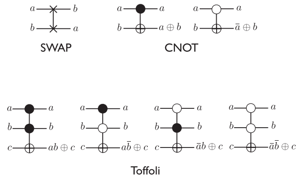
FIG. 1. Reversible gates used in the quantum stochastic evolutions. The output values of the gates are defined when a , b , and c take values 0 and 1. Top row: The two-qubit gates SWAP and CNOT. Bottom row: The different variations of the three-qubit Toffoli gates. We note that different variations of the CNOT and Toffoli gates can be obtained from one fixed variation plus NOT gates.
