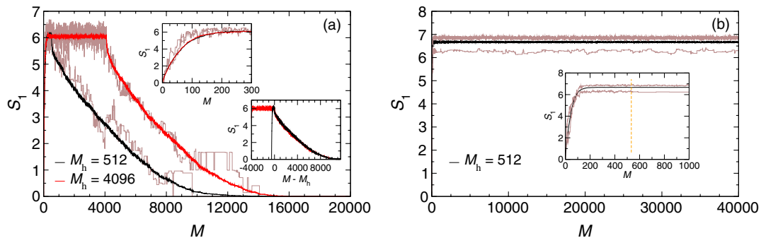
FIG. 2 (color online). Evolution of the entanglement entropy S_1 obtained from the bipartition of the qubit string at the middle ( n_A = n_B = 8 ) as a function of the number of applied gates. First, M_h reversible gates are randomly applied (heating period); second, a Metropolis algorithm is used to reverse the evolution and restore zero entropy (cooldown period). The shorter solid black line ( M_h = 512 ) and the longer red line ( M_h = 4096 ) result from averaging S_1 over 128 initial-state realizations. The faded brown lines show the evolution of S_1 for two typical realizations. (a) Only two-qubit gates are used. Upper inset: The heating period. Lower inset: Shifted curves, showing that the cooling, on average, is independent of the duration of the heating period. (b) A mixture of two-qubit and Toffoli gates is used. Inset: Detail of the transition between heating and cooling periods. The dashed line indicates the transition point.
