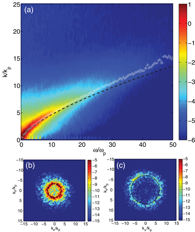
FIG. 2 (color online). (a) S_\eta(\omega/\omega_p, k/k_p) . Key to symbols: (dashed line) linear dispersion relation \omega^2 = (\gamma/\rho)k^3 ; (white crosses) spectrum maxima. S_\eta(k_x/k_p, k_y/k_p) at a fixed \omega^* = \omega/\omega_p = 6 (b) and \omega^* = \omega/\omega_p = 18 (c). Circles in solid line indicate k^*(\omega^*) given by the dispersion relation. The wave field is found isotropic. Colors are S_\eta log scaled.
