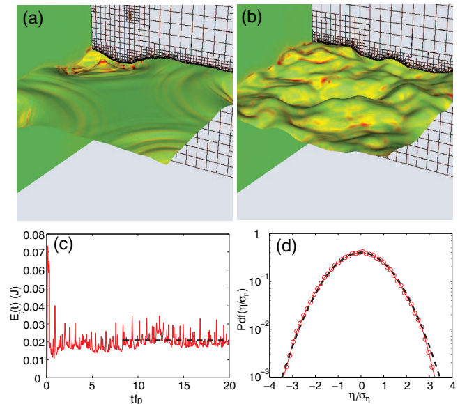
FIG. 1 (color online). Snapshot of the wave interface \eta(x, y) at time tf_p = 0.3 (a) and tf_p = 9.1 (b). (c) Total wave energy E_t as a function of time tf_p . A stationary state is reached for tf_p > 5 , and the mean value is indicated by the dashed line. (d) PDF of the wave height \eta/\sigma_\eta . Dashed line is the normalized Gaussian.
