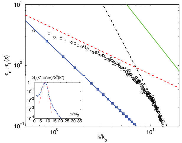
FIG. 4 (color online). Time scale evolutions as a function of k/k_p . Key to symbols: ( \circ ), \tau_{nl}(k) = 1/\Delta\omega ; ( \blacksquare with line), \tau_l = 1/\omega ; (solid line), \tau_d = 1/(2\nu k^2) viscous dissipation; and (dot-dashed line), \tau_d^{\text{num}} numerical dissipation function ( 1/\tau_d^{\text{num}} = \mathcal{A}(k/k_{\text{max}})/\tau_d , with \mathcal{A} \approx 100 an empirical nondimensional parameter; see Supplemental Material [35]). Theoretical prediction \tau_{nl} \sim k^{-3/4} (dashed line). Inset: S_\eta(k^*, \omega) normalized by its maximum S_\eta^0(k^*) as a function of \omega/\omega_p , for k^*/k_p = 7.6 . Gaussian fit (dashed line), \exp[-(\omega - \omega_c)^2/\Delta\omega^2] with \Delta\omega = 2\pi 0.15 and \omega_c = 2\pi 0.66 \text{ rad}^{-1} .
