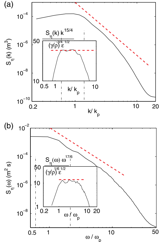
FIG. 3 (color online). (a) S_\eta(k/k_p) . (b) S_\eta(\omega/\omega_p) . Theoretical KZ spectrum (dashed line) is respectively S_\eta \sim k^{-15/4} and S_\eta \sim \omega^{-17/6} . Inset: compensated spectrum, respectively S_\eta(k)(k)^{15/4}/[\epsilon^{1/2}(\gamma/\rho)^{-3/4}] and S_\eta(\omega)\omega^{17/6}/[\epsilon^{1/2}(\gamma/\rho)^{1/6}] . Vertical dot-dashed line indicates the forcing scale range.
