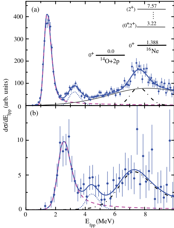
FIG. 3 (color online). (a) The ^{14}\text{O} + p + p relative-energy spectrum used to verify the experimental resolution and the energy calibration (see Table I). The thin solid line extending below the spectrum is due to a nonresonant background. (b) The ^{13}\text{O} + p + p relative-energy spectrum. The spectra are decomposed into several Breit-Wigner-shaped resonances convoluted with the experimental resolution.
