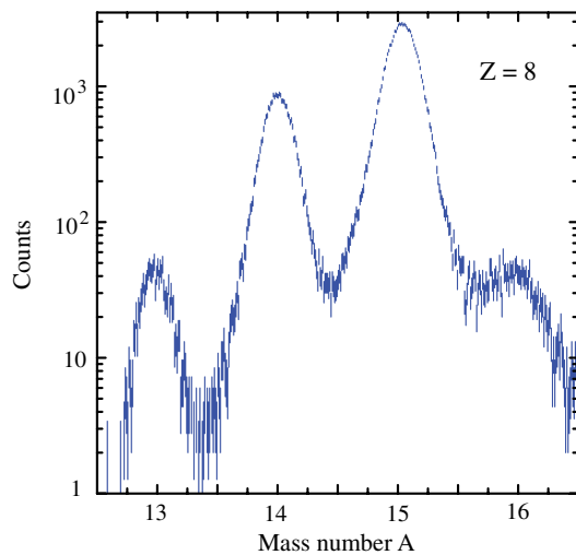
FIG. 1 (color online). Mass identification plot for final-state oxygen isotopes produced in the breakup of 500 MeV/u ^{17}\text{Ne} projectiles on carbon and polyethylene targets.
