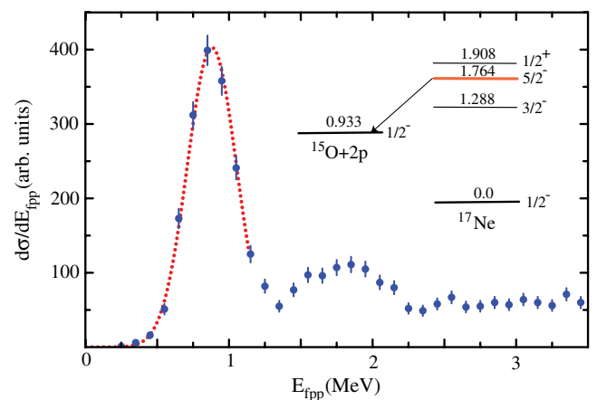
FIG. 2 (color online). The ^{15}\text{O} + p + p relative-energy spectrum. The intense peak corresponding to the known ^{17}\text{Ne}(5/2^-) state at an excitation energy of 1.764 MeV was used as benchmark for the experimental E_{fpp} resolution and for the fine-tuning of the energy calibration. The dotted line represents a Gaussian fit.
