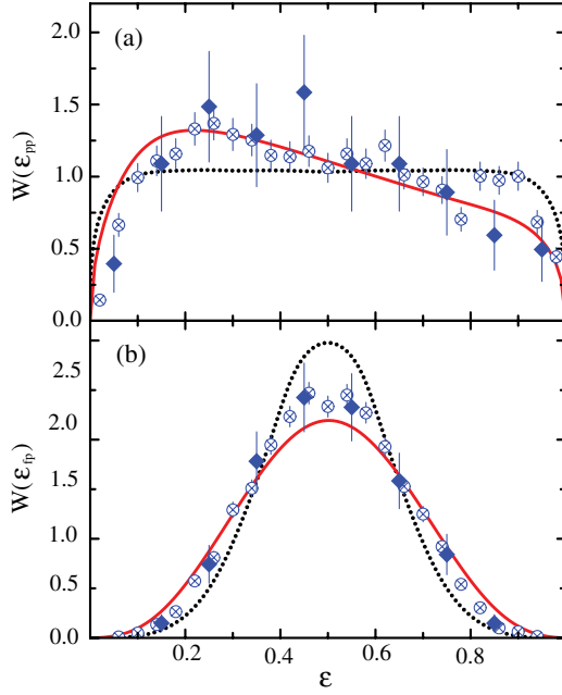
FIG. 5 (color online). Fractional energy spectra for ^{15}\text{Ne} (diamond) and ^{16}\text{Ne} (crossed circle). The distribution on fractional relative energy (a) between two protons and (b) between one proton and a ^{13,14}\text{O} fragment for ^{15,16}\text{Ne} , respectively, are shown as distributions normalized to unity. The solid lines are the results of theoretical calculations within a three-body model in the case of ^{16}\text{Ne} [19]. The dotted lines show the result of a calculation assuming sequential decay of ^{15}\text{Ne} via the ground state of ^{14}\text{F} .
