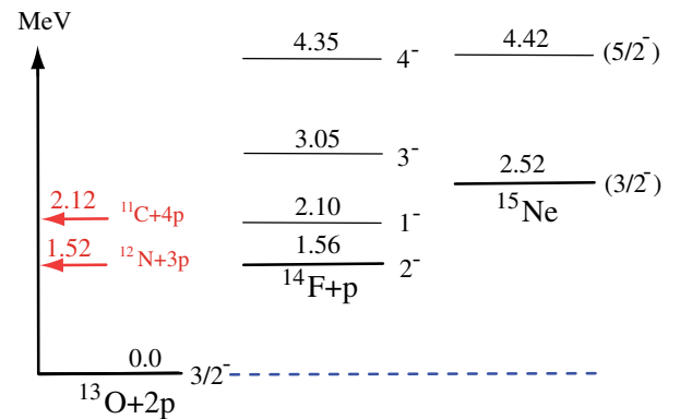
FIG. 4 (color online). Level schemes for ^{15}\text{Ne} and daughter nuclei. The energies are given from zero internal energy in the ^{13}\text{O} + p + p system. Thresholds for few-body decays are also shown. The energy levels for ^{14}\text{F} are taken from Ref. [18].
