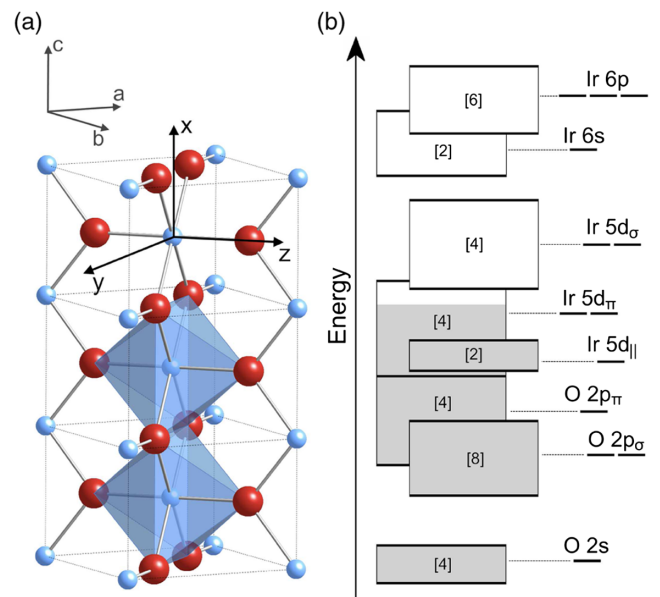
FIG. 4 (color online). (a) The rutile crystal structure of the iridium-centred unit cell with the x , y , and z coordinates defined. (b) Schematic description (Goodenough model [33]) of the electronic structure of \text{IrO}_2 .
