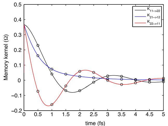
FIG. 4 (color online). Real parts of nonzero elements of the memory kernel as a function of time. The nonzero elements are \mathcal{K}_{11\rightarrow 11} = -\mathcal{K}_{11\rightarrow 22} , \mathcal{K}_{22\rightarrow 22} = -\mathcal{K}_{22\rightarrow 11} , and \mathcal{K}_{12\rightarrow 21} = -\mathcal{K}_{21\rightarrow 21} = -\mathcal{K}_{12\rightarrow 12} = \mathcal{K}_{21\rightarrow 12} . The solid lines represent the matrix elements of the memory kernel extracted by applying TTM to a hierarchy simulation of a symmetric two-level system with coupling \Omega . The dots are the values corresponding to the analytical prediction. The dissipative system is characterized by the parameters \lambda = 0.25 \Omega , \gamma = 0.05 \Omega , and \beta\Omega = 4.79 .
