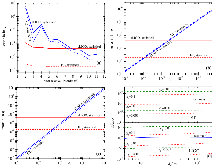
FIG. 2 (color online). aLIGO and ET statistical and systematic parameter errors for different waveform approximations. (a) Fractional errors in \eta due to neglecting high PN-order terms as a function of the relative PN order in \Psi_{AP} . (b) The corresponding error due to neglecting spin effects. (c) The error from neglecting orbital eccentricity. (d) The ratio of systematic to statistical errors in the reduced tidal deformation parameter \tilde{\Lambda} as a function of \hat{\lambda}_i and for different waveform errors (neglecting spin, eccentricity, or high PN terms). All plots are for a m_1 = m_2 = 1.4M_\odot BNS at 100 Mpc. Angle-averaged SNRs are 14.5 for aLIGO and 175 for ET. These results are relatively insensitive to small changes in \eta that keep M constant.
