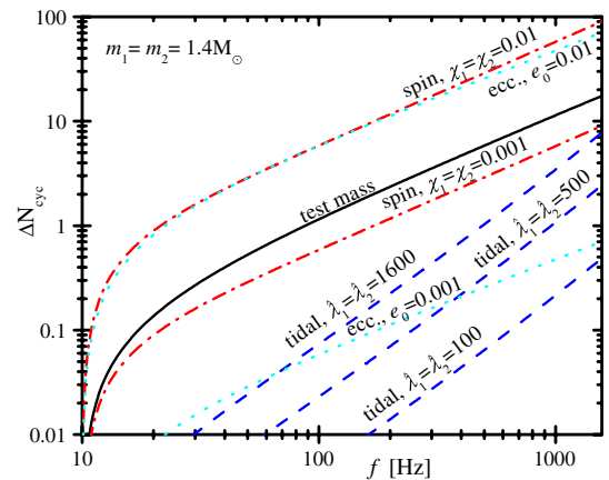
FIG. 1 (color online). Contribution of the last four terms in Eq. (1) to the number of wave cycles in the phase of the Fourier transform \tilde{h}(f) . Parameter values are as indicated; t_c and \phi_c are chosen such that \Delta N_{\text{cyc}} and its frequency derivative vanish at a reference frequency f_0 = 10 Hz: i.e., for each term X , 2\pi\Delta N_{\text{cyc}}^X = \Delta\Psi^X(f) - \Delta\Psi^X(f_0) + (f - f_0)d\Delta\Psi^X/df_0 , where \Delta\Psi^X \equiv 3\Delta\Psi^X/(128\eta v^5) .
