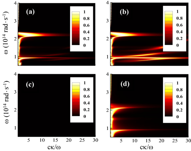
FIG. 2 (color online). Transmission probabilities of energy carried by the modes. Efficiency of coupling of modes (\omega, \kappa) in a \text{SiO}_2 - \text{VO}_2 - \text{SiO}_2 system ( \delta = 50 nm and d = 100 nm). (a) T_p^{S/G} and (b) T_p^{G/D} with \text{VO}_2 in its crystalline state. (c) T_p^{S/G} and (d) T_p^{G/D} with \text{VO}_2 in its amorphous state. Wien's frequency (where the transfer is maximum) at T = 340 K is \omega_{\text{Wien}} \sim 1.3 \times 10^{14} rad/s. The dielectric permittivity of \text{SiO}_2 is taken from the database [19].
