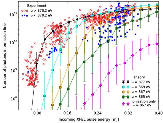
FIG. 5 (color online). Pump-energy dependence of the SRXRS signal: measured number of photons in the emission line as a function of the incoming pulse energy for \omega > 870 eV (average \bar{\omega} = 876 eV) and \omega < 870 eV ( \bar{\omega} = 868 eV) along with the theory results for \omega = 877 , 869, 867, and 865 eV. Each data point of the theory results corresponds to the geometric mean and standard deviation of 50 SASE pulses.
