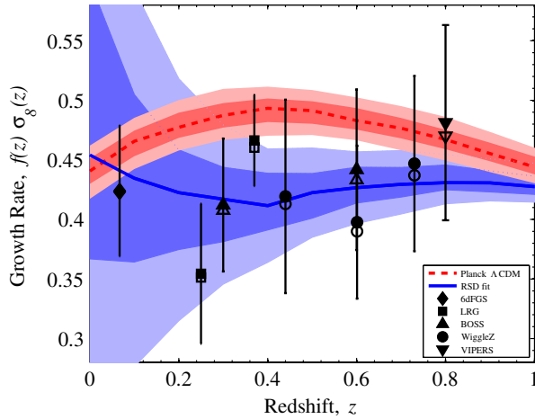
FIG. 1 (color online). Comparing models to recent measurements of f(z)\sigma_8(z) . We are plotting results for the \text{LRG}_{200} data set. The open markers are the original published values from the RSD measurements, and the filled markers are after accounting for the Alcock-Paczynski effect in going from WMAP to Planck cosmology. The measurement error bars are at the 1 standard deviation uncertainty level. The dashed red line illustrates the expected growth rate from \Lambda\text{CDM} with Planck parameters, with the 1 and 2 standard deviation uncertainty illustrated with the shaded bands. The solid blue line and corresponding blue shaded regions illustrates the best fit to the RSD data with the gravitational slip model. We note that almost all the measurements include our best fit model at the 1 standard deviation uncertainty level, which is reflected in the low \chi^2 in Table II. The 1 standard deviation range of the model (the darker blue band) is narrower than the typical 1 standard deviation uncertainty on any of the measurements because the fit has been calculated from the several independent measurements.
