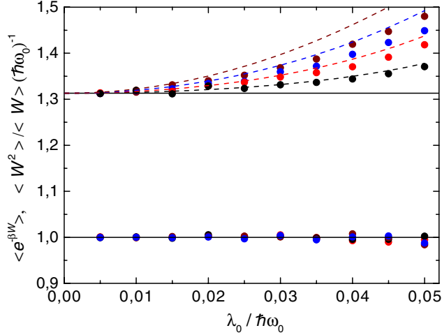
FIG. 3 (color online). Results of numerical simulations and analytic approximations. The ratio of the two lowest moments of work and the JE average are shown as functions of the driving amplitude. The symbols are numerical simulations and the lines are analytical approximations; the colored ones are for the perturbative in \Gamma_{\downarrow, \uparrow} calculation. Here, \beta \hbar \omega_0 = 2.0 , the resonant ( \omega = \omega_0 ) drive lasts 10 cycles, and the various data sets are for \Gamma_1 = (0, )0.005, 0.01, 0.015, 0.02 from bottom to top.
