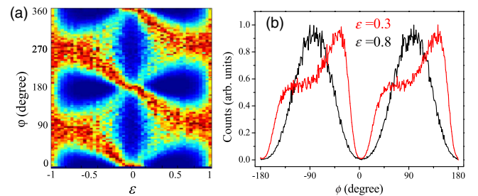
FIG. 5 (color online). (a) The simulated ellipticity-dependent momentum-integrated angular distribution for He. (b) The simulated angular distributions for two ellipticity values. In the simulation, there is no initial longitudinal momentum included.
