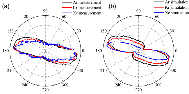
FIG. 4 (color online). The experimental (a) and simulated (b) momentum-integrated angular distributions of Ar, Kr, and Xe (ellipticity \sim 0.25 ) at an intensity of 1.5 \times 10^{14} W/cm ^2 .
