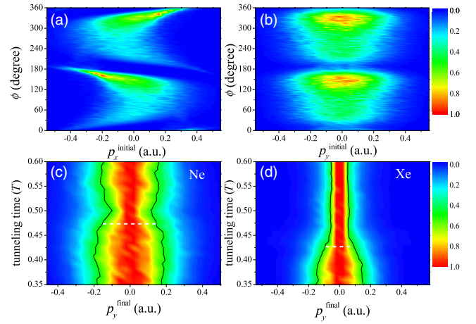
FIG. 3 (color online). (a) and (b) show the momentum-integrated angular distributions with respect to the initial transverse velocities of along the minor axis and the laser propagation direction. (c) and (d) show the electron tunneling time with respect to the final transverse momentum along the laser propagation direction (c) for Ne 3 \times 10^{14} W/cm 2 and (d) for Xe 1.5 \times 10^{14} W/cm 2 (the ellipticity \sim 0.25 ). The solid lines and dashed lines in (c) and (d) show the position of half maximum of p_y^{\text{final}} and the tunneling time when rescattering begins to occur, respectively, and the color scale is normalized to the maximum rate for each tunneling time.
