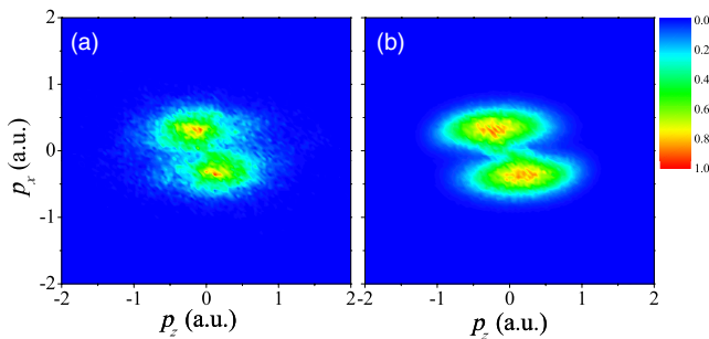
FIG. 1 (color online). The two-dimensional experimental (a) and simulated (b) photoelectron momentum distributions of Ne in an elliptically polarized laser field at an intensity of 3 \times 10^{14} W/cm 2 .
