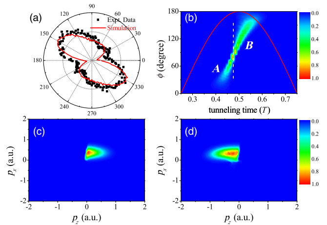
FIG. 2 (color online). (a) The momentum-integrated angular distribution of Ne in an elliptical laser field (the ellipticity \sim 0.25 ) at an intensity of 3 \times 10^{14} W/cm 2 of experiment (dotted) and simulation (solid). (b) The momentum-integrated angular distribution with respect to the tunneling time. The red solid line shows the field component along the major axis. Two groups of electrons marked A and B are mainly induced by direct ionization and multiple forward scattering, which are separated by the white dashed line. (c) and (d) show two-dimensional photoelectron momentum distributions of direct ionization and multiple forward scattering, respectively.
