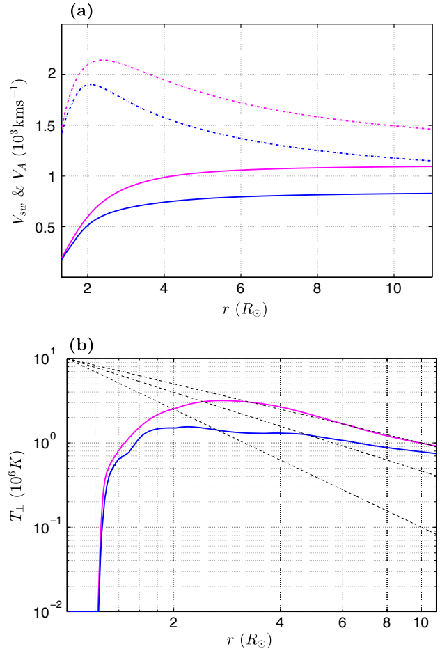
FIG. 1 (color online). The radial dependence of (a) the proton streaming speed U_{sw} (solid line) and the Alfvén speed v_A (dashed line), and (b) the proton perpendicular temperature T_\perp in the coronal hole (bottom blue lines correspond to \sim 20\text{--}25 \text{ km s}^{-1} injection wave amplitudes; upper magenta lines to infinite wave energy flux). Dashed lines in (b) show theoretical scalings for CGL expansion ( r^{-2} ), for collisional expansion ( r^{-4/3} ), and for kinetic resonance sweeping cooling ( r^{-1} ).
