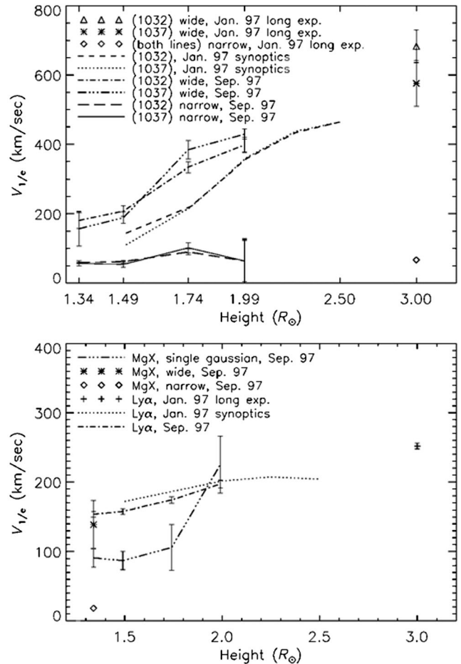
FIG. 3. The line width components expressed as velocities for O^{5+} ions (top) and Mg^{9+} ions (bottom) as a function of height (adopted from [4], Fig. 3).
