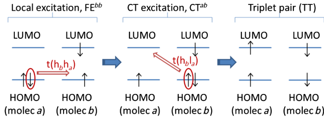
FIG. 2 (color online). Schematic one-electron energy diagram showing single Frenkel, charge-transfer and triplet pair excitations in a localized representation of a molecular dimer \{a, b\} . The labels in red refer to the resonance integrals coupling these electronic configurations, see text.
