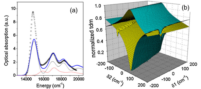
FIG. 3 (color online). (a) Calculated absorption spectra along with experiment spectra ( \square ) of Sebastian et al. [21]. The black and red curves represent respectively \parallel b and \perp b polarized spectra and the blue curves represent unpolarized spectra. Experiment and the calculated spectra are normalized and aligned at the 0–1 peak. (b) Transition dipole moment (tdm) as a function of the disparities in CT energies ( \delta 1 ) and matrix elements ( \delta 2 ). The top surface represents the highest tdm among the coupled FE/TT states while the bottom surface represents second largest tdm. Note that at (0, 0), there is no tdm sharing between the FE and the TT states due to cancellation effects.
