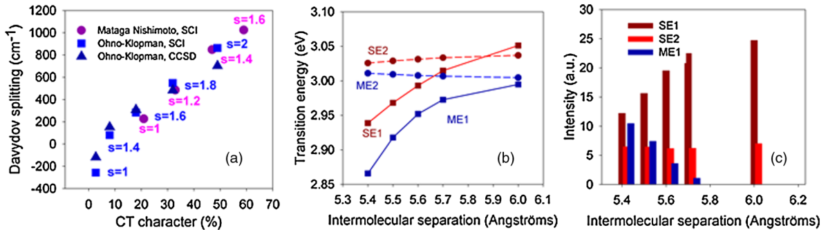
FIG. 1 (color online). (a) Davydov splitting calculated at the INDO/SCI and INDO/CCSD levels versus the charge-transfer character in the lowest eigenstate of a pentacene unit cell dimer. The results are shown for two different electron-electron potentials V(r) and using different screening factors s , with V_{\text{scr}}(r) = V(r \times s) . (b) INDO/CCSD ( s = 1.4 ) transition energies to the lowest three singlet excited states of the pentacene unit cell dimer versus intermolecular separation. SE1 and SE2 denote single exciton states (their energy difference is the DS) and ME1 is a double exciton state. (c) Relative intensities (squared transition dipole moment) for the lowest three electronic transitions in Fig. 1(b). Note the strong intensity borrowing from SE1 to ME1 at short distances.
