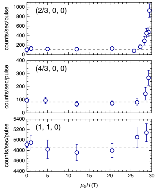
FIG. 3 (color online). Magnetic field dependence of the intensity at the (2/3, 0, 0) and (4/3, 0, 0) magnetic Bragg peaks and at the (1,1,0) nuclear Bragg peak at 1.7 K. The intensity of neutron counts is averaged over increasing and decreasing fields. The vertical red dashed lines correspond to the critical field \mu_0 H_C = 26 T. The horizontal dashed lines represent the background intensity.
