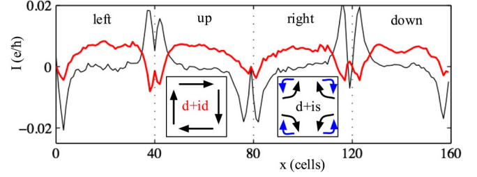
FIG. 3 (color online). Disorder averaged surface currents in the clockwise direction summed over the ten first surface layers on each of four sides (left, up, right, down) for L = 40 and T_{c,d_2} = 0.5T_c (thick red line) and T_{c,s} = 0.5T_c (black line). Vertical dashed lines mark the corners. Insets show schematically the surface current orientation. Black arrows indicate currents present after disorder averaging, blue (gray) arrows indicate outermost surface currents prone to cancellation in disorder averaged results.
