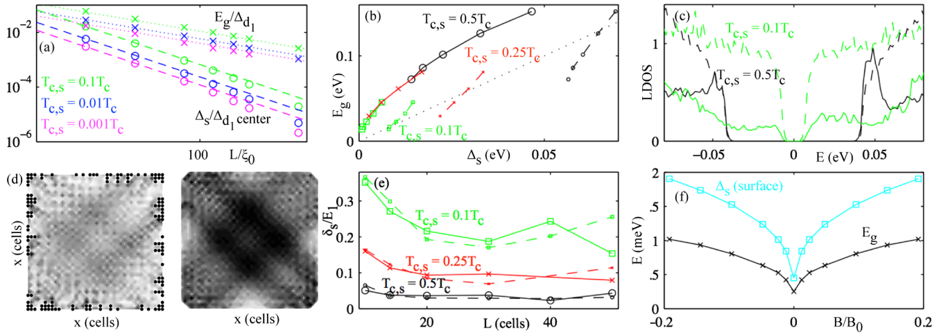
FIG. 1 (color online). Subdominant s -wave order. (a) QC s -wave component \Delta_s in the center of the island (circles) and nodal energy gap E_g (times) of a pair-breaking [110] surface with disorder as a function of slab length L/\xi_0 for T_{c,s}/T_c = 0.001 (magenta), 0.01 (blue), 0.1 (green) (increasing values) at temperature T = 0.01T_c . Dashed lines are \Delta_s(\text{center}) = 48\Delta_s(\text{surface})/[1 - \log(T_{c,s}/T_c)](L/\xi_0)^2 , dotted lines are E_g = 4\Delta_s(\text{surface})/(L/\xi_0) . (b) BdG disorder averaged energy gap E_g as a function of \Delta_s in the center of the grain (solid) and at the surface (dashed) for T_{c,s} = 0.5T_c (black, circles), 0.25T_c (red, crosses), and 0.1T_c (green, squares). Dotted line is E_g = 2\Delta . (c) BdG disorder averaged LDOS in the center of the grain (solid line) and at the surface (dashed line). (d) BdG eigenstate spatial density for one disorder configuration with L = 40 (black dots marking removed sites) averaged over the four lowest energy states (left) and disorder averaged (40 configurations) for the lowest energy state (right). White = zero, black = 0.01 (left) or 0.005 (right) states per unit cell. (e) BdG disorder averaged level spacing \delta_s = E_{n+1} - E_n ratio to first energy value E_1 for n = 1 (solid lines) and n = 2 (dashed lines) as a function of grain size L . (f) Evolution of the QC energy gap E_g (black, crosses) and \Delta_s on the surface (cyan, squares) with magnetic field, B_0 = \Phi_0/\pi\xi_0\lambda_0 \approx 2.2 T (derived assuming \xi_0 = 2 nm, \lambda_0 = 150 nm for YBCO) for a L = 40\xi_0 slab with surface disorder modeled by a thin layer ( \sim 0.2\xi_0 ) with a graded impurity concentration [32] and T_{c,s} = 0.065T_c .
