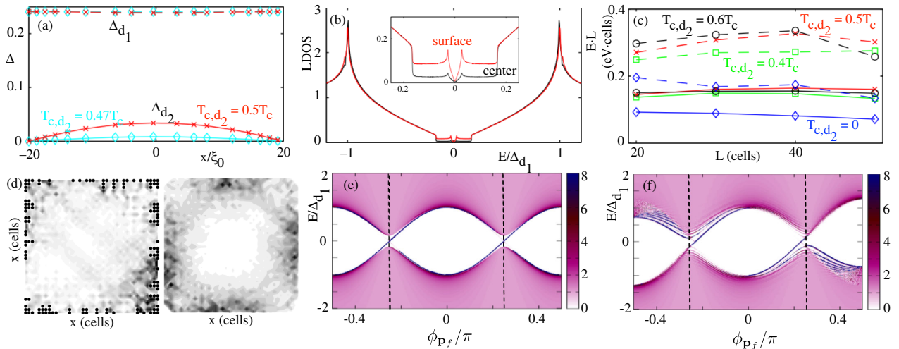
FIG. 2 (color online). Subdominant d_2 -wave order. (a) QC d_1 -wave (dashed line), and d_2 -wave (solid lines) components across a L = 40\xi_0 [100] slab for T_{c,d_2} = 0.5T_c (red, crosses) and 0.47T_c (cyan, diamonds). (b) QC LDOS in units of normal state LDOS in the center (black line) and at the surface (red line). Inset shows a zoom-in at low energies. (c) BdG energy eigenstates times grain size L as a function of L for E_1 (solid lines) and E_2 (dashed lines) for T_{c,d_2} = 0.6T_c (black, circles), 0.5T_c (red, crosses), 0.4T_c (green, square), and 0T_c (blue, diamonds). (d) Same as Fig. 1(e) but for d_2 -wave order. (e), (f) QC band structure at the surface for B = 0 (e) and B = 2B_0 (f) with color scale showing the angle resolved LDOS, i.e., \phi_{P_f} measures the position on the Fermi circle measured from the k_x -axis. Dashed lines mark the d_1 node.
