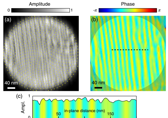
FIG. 2 (color online). (a) The amplitude of the BPP reconstructed PbTiO 3 thin film projection is shown in grayscale along with the raster positions of the beam (yellow dots). (b) The corresponding phase of the reconstruction. (c) A line through the reconstruction [along the dotted line in (b)] plotting reconstructed object amplitude colored by the corresponding pixel phase.
