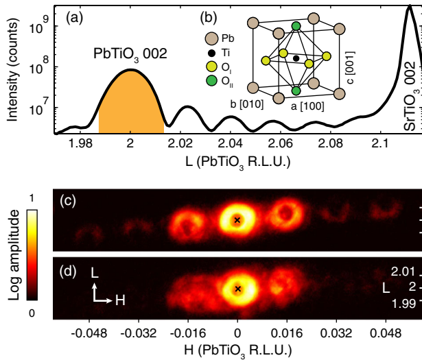
FIG. 1 (color online). (a) The 00 L CTR containing the 002 Bragg peaks of the PbTiO 3 film and the underlying SrTiO 3 substrate measured with an unfocused x-ray beam. The shaded region of the PbTiO 3 peak corresponds to the angular divergence of the zone plate focusing optic. (b) The cubic perovskite PbTiO 3 unit cell structure. (c), (d) Coherent diffraction patterns taken with the focused beam illuminating 180° ferroelectric stripe domains. The x marks the position of the PbTiO 3 Bragg peak (10 s exposures).
