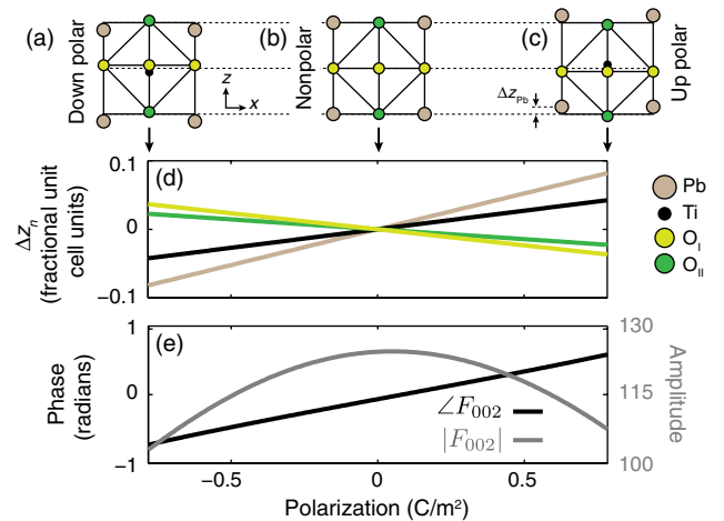
FIG. 3 (color online). The unit cell structures of PbTiO 3 corresponding to fully compensated bulk polarization in the (a) “down” and (c) “up” states are shown as they appear relative to each other across a 180° domain wall, as calculated from ab initio theory [29]. (b) The centrosymmetric reference structure. The ionic displacements \Delta z_n and the unit cell structure factor F_{002} are plotted vs polarization in (d) and (e).
