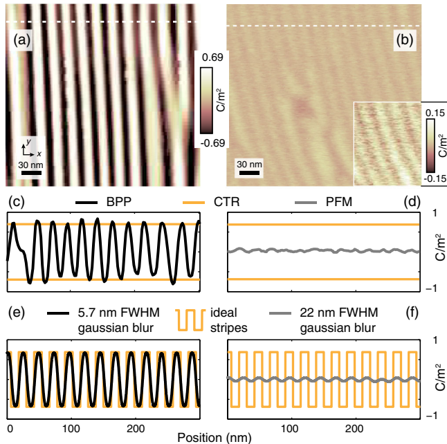
FIG. 4 (color online). (a) The stripe domain polarization map generated from the phase of the BPP reconstruction is shown, along with a polarization map measured with PFM in (b). The images show different regions of the sample but share the central color scale [with the exception of the inset in (b), which uses the right-hand scale]. Profiles taken along the white dotted lines in each image are plotted below the corresponding image in (c) and (d). The horizontal lines in (c)–(f) represent the average polarization state of the film ( \pm 0.69 \text{ C/m}^2 ) as determined from the CTR. By fitting such line profiles, the spatial resolutions of these BPP and PFM measurements were determined to be 5.7 and 22 nm, and the effect of these resolution functions on idealized stripe domains with \Lambda = 23 \text{ nm} is shown in (e) and (f).
