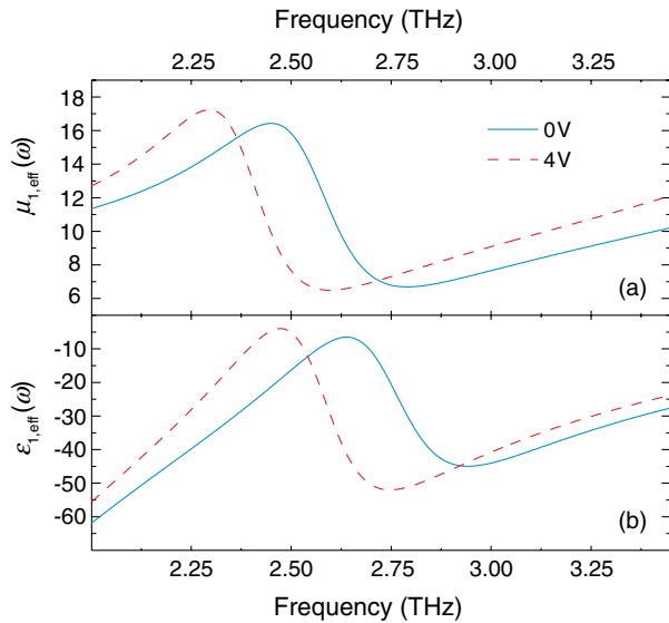
FIG. 5 (color online). Effective optical constants of metamaterial absorber. (a) Real part of effective permeability ( \mu_{1,\text{eff}} ), and (b) real part of effective permittivity ( \epsilon_{1,\text{eff}} ), determined from inversion of the simulated scattering parameters for 0 V (blue solid curves) and 4 V (red dashed curves).
