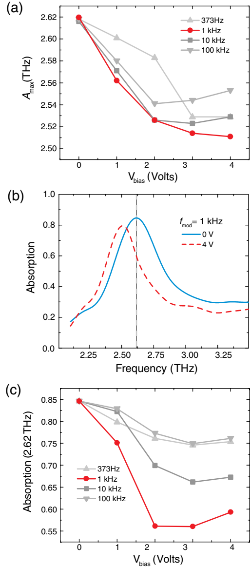
FIG. 2 (color online). Experimentally measured absorption of the metamaterial absorber. (a) Frequency location of the absorption maximum ( A_{\text{max}} ) as a function of applied bias voltage ( V_{\text{bias}} ) for modulation frequency ( f_{\text{mod}} ) values of 373 Hz, 1 kHz, 10 kHz, and 100 kHz. (b) Frequency dependent absorption A(\omega) for 0 V (blue solid curve) and 4 V (red dashed curve) at f_{\text{mod}} = 1 kHz, dashed line is centered at A_{\text{max}}(V_{\text{bias}} = 0) = 2.62 THz. (c) The absorption value at 2.62 THz as a function of V_{\text{bias}} for various modulation frequencies.
