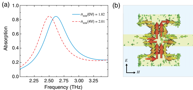
FIG. 3 (color online). Numerical simulations of the metamaterial absorber. (a) THz absorption simulated for 0 V (blue solid curve) and 4 V (red dashed curve) at f_{\text{mod}} = 1 kHz. (b) Simulated current density in the ERR for the case of the unbiased absorption maximum A_{\text{max}}(V_{\text{bias}} = 0) = 2.62 THz.
