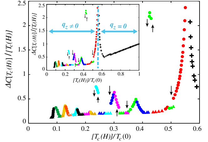
FIG. 3 (color online). Specific heat jump at the onset of the modulated SC order in field \Delta C[T_c(H)]/T_c(H) . The notations are the same as in Fig. 2. Inset: the same over the entire temperature range of the superconducting transition. The nonmonotonic behavior appears only for the FFLO state, q_z \neq 0 .
