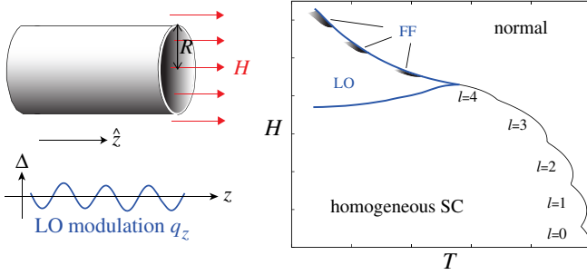
FIG. 1 (color online). Left: Superconducting thin-wall cylinder with a small radius R in a magnetic field parallel to the cylinder axis ( z axis). Sketch shows the spatial modulation of the order parameter in the LO phase. Right: Phase diagram in the H - T plane, showing regions of the normal phase, homogeneous ( q_z = 0 ) superconductor, and spatially modulated LO phase, with phase-modulated FF states indicated by the shaded regions.
