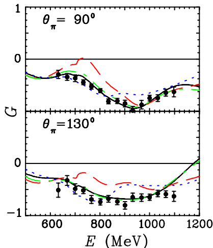
FIG. 1 (color online). Double-polarization observable G for \gamma p \rightarrow \pi^0 p as a function of energy for two selected bins in \theta_\pi . Curves: solid (black): BG2011-02 of BnGa [2], dashed (red): SN11 of SAID [5], dash-dotted (green): CM12 of SAID [4], and dotted (blue): MAID07 [3]. Black dots show CB-ELSA/TAPS Collaboration data [1]. Plotted uncertainties are statistical.
