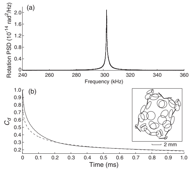
FIG. 2. (a) Unpolarized atom spin noise spectrum taken at 0.42 G with atom density of 1.2 \times 10^{13}/\text{cm}^3 after subtraction of the photon shot noise background from a spin noise measurement at low magnetic field. (b) Spin correlation function due to the diffusion of the atoms out of the probe beam. Solid line (dashed line) is the experimental (calculated) result with atom density of 1.2 \times 10^{13}/\text{cm}^3 . The inset shows the calculated beam pattern at the center of the cavity.
