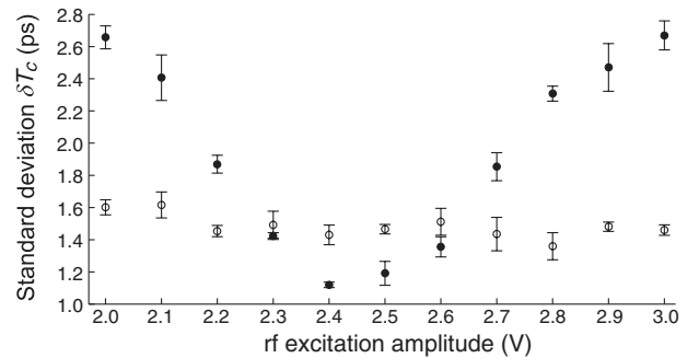
FIG. 3. The dependence of the standard deviation \delta T_c on the rf pulse amplitude. Empty (solid) circles denote the backaction evasion with stroboscopic modulation (normal modulation) of probe light. Here the probe pulse length and T are equal to four Larmor periods.
