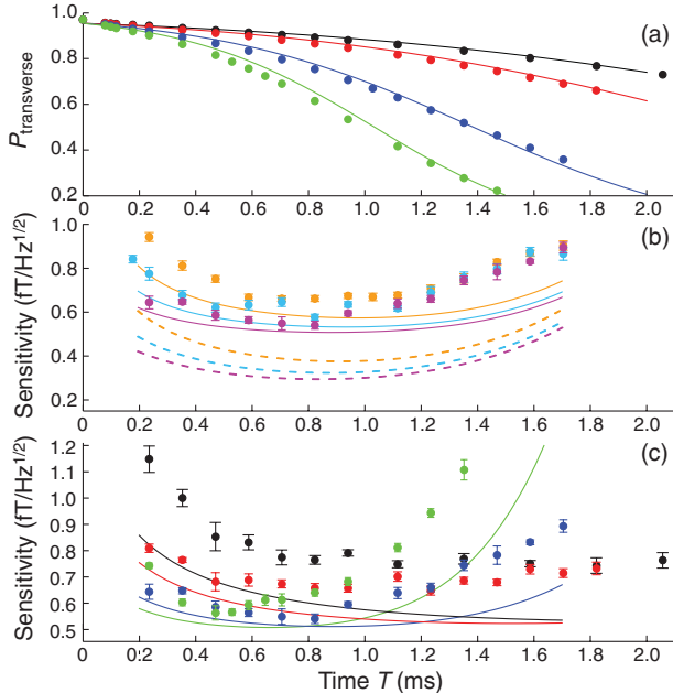
FIG. 4 (color). (a) Relaxation of transverse polarization P_t (points) for n = 1.9 (green), 1.4 (blue), 0.8 (red), and 0.6(\text{black}) \times 10^{13}/\text{cm}^3 together with theoretical prediction (lines). (b) The points are the experimental results of magnetic field sensitivity at n = 1.4 \times 10^{13}/\text{cm}^3 , with probe pulse length of 4 (orange), 8 (cyan), and 12 (purple) Larmor periods. Solid (dashed) lines are the theoretically calculated sensitivity based on measured parameters with (without) magnetic shield noise and time jitter noise. (c) Experiment results (points) of magnetic field sensitivity with probe length of 12 Larmor periods at different atom densities, with the same color notation as plot (a), together with theoretical predictions (lines).
