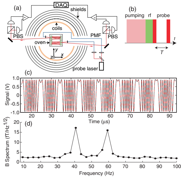
FIG. 1 (color online). (a) Experiment setup. PBS: polarization beam splitter; PMF: polarization maintaining fiber; DAQ: data acquisition card. (b) The timing of the pulsed operation. (c) Optical rotation (black line) recorded for one probe pulse at atom density of 0.8 \times 10^{13}/\text{cm}^3 together with a fitted curve (red dashed line). (d) Magnetic field noise spectrum obtained in the gradiometer in the presence of a calibrating magnetic field gradient at 40 Hz. The peak at 60 Hz is due to ac line noise.
