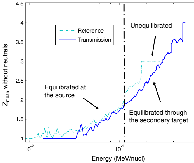
FIG. 2 (color online). Z_{\text{mean}} for carbon ions as measured by the “reference” TP1 and “transmission” TP2 after 100 nm of aluminum target at 300 K. The error is \pm 0.005 MeV/nucleon for the energy and the uncertainty is \pm 0.1 for the mean charge.
