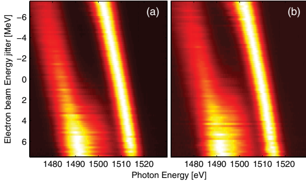
FIG. 4 (color online). Results for two-color beams with scheme II. (a),(b) Average spectral intensity as a function of the electron beam energy and photon energy. For each electron beam energy, the maximum intensity has been normalized to 1. (a) 21 fs delay. (b) 26 fs delay.
