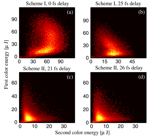
FIG. 5 (color online). Shot-to-shot intensity correlation between first and second color generated in the Two-Color schemes. Each spectrum has been fit with a sum of two Gaussians, and the energy is considered proportional to the fit area. (a) scheme I with 0 fs delay, (b) scheme I with 25 fs delay, (c) scheme II with 21 fs delay, and (d) scheme II with 26 fs delay.
