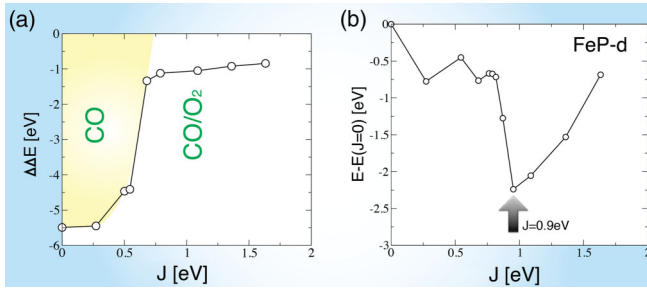
FIG. 3 (color online). Energetics. (a) Difference in CO and O 2 binding energies \Delta\Delta E . The binding to CO is always favored; however, the imbalance is strongly reduced for J > 0.5 eV. (b) Total energy of FeP as a function of J . The minimum of the total energy is obtained for J = 0.9 eV.
