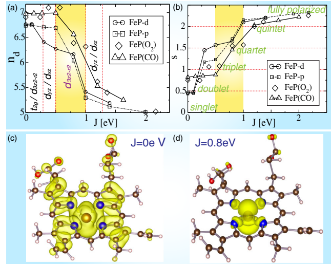
FIG. 1 (color online). Orbital selection process. Dependence of (a) the iron 3d subspace occupancy n_d and (b) the effective spin quantum number s on the Hund's coupling J , for both unligated and ligated heme models. The physically relevant region 0.5 < J < 1 eV is highlighted in light gray (yellow). Isosurfaces of the real-space representation of the electronic spectral density of the HOMO of FeP- d for (c) J = 0 eV and (d) J = 0.8 eV. The large central sphere shows the location of the iron atom, and the four dark gray (blue) spheres indicate nitrogen atoms.
