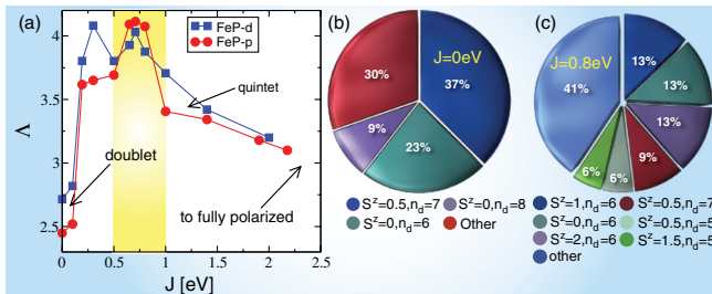
FIG. 2 (color online). Valence fluctuations. (a) von Neumann entropy \Lambda obtained by DFT + DMFT for FeP- p (circles) and FeP- d (squares). The dominant electronic configurations for FeP- d for (b) J = 0 eV and (c) J = 0.8 eV. The pie wedge labeled other contains configurations with a weight smaller than 3%. The iron 3d spin S^z and iron 3d occupancy n_d of the dominant configurations are indicated.
