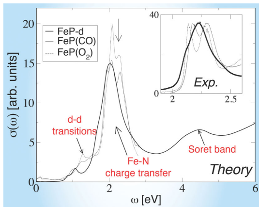
FIG. 4 (color online). Optical response. Optical conductivity of FeP- d (bold line), FeP(CO) (solid), and FeP(O 2 ) (dashed line). The vertical arrow indicates the energy of the experimental peak associated with the Fe-N charge transfer. Inset: Experimental measurements [28] for unligated heme (bold line), oxyheme (dashed line) and carboxyheme (solid) are shown for comparison. J = 0.8 eV was used for these calculations.
