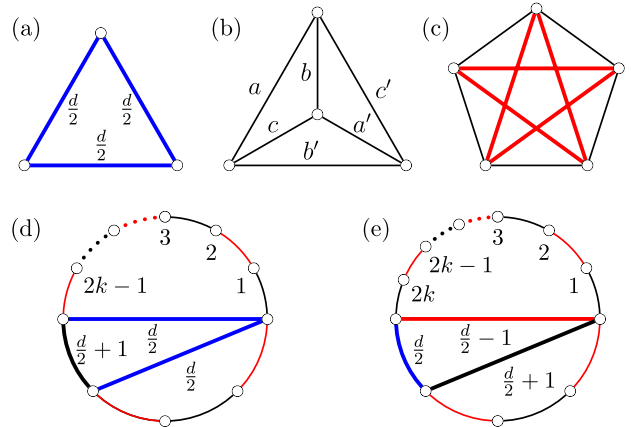
FIG. 1 (color online). Examples of GHZ graphs. Unlabeled thin black or red edges have weight 1 or d-1 , respectively. All possible GHZ graphs on 3 and 4 vertices are shown in (a) and (b), where a' = \frac{d}{2} + a, b' = \frac{d}{2} + b , and c' = \frac{d}{2} + c with a + b + c = d/2 . A GHZ graph on 5 vertices is shown in (c) where the thick red edges have weight d/2 - 1 . In (d) and (e) two primary GHZ graphs on 2k + 4 and 2k + 5 vertices ( k \geq 1 ) are shown.
