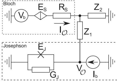
FIG. 1. A general linear circuit embedding a phase-slip (diamond) and a Josephson (cross) junction illustrates the problem of quantum synchronization of the circuit parts (dashed boxes) that generate Bloch and Josephson oscillations. The parts are coupled by the (frequency-dependent) resistors Z_1 and Z_2 . The circuit is controlled with voltage and current sources V_b, I_b and provides current and voltage outputs V_O, I_O . The solution to the problem is presented in Fig. 2.
