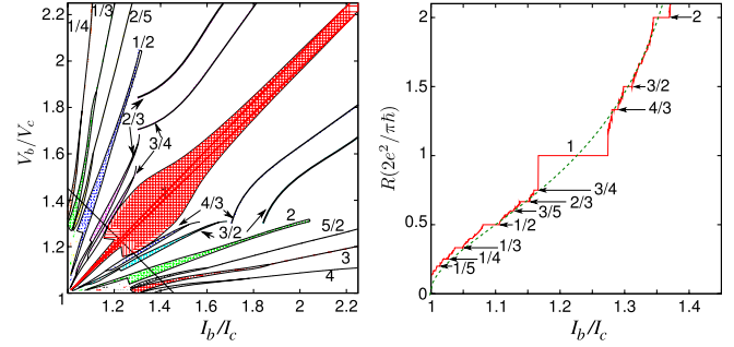
FIG. 3 (color online). Left: Synchronization domains ( n/m ) in the plane of normalized bias voltage and bias current. Right: Quantized plateaus of transresistance R = V_O/I_O along the cut given by the line in the left-hand figure. Dashed curve: Continuous transresistance as set by uncoupled Bloch and Josephson parts, R = (\pi\hbar/2e^2)\bar{\omega}_J(I_b)/\bar{\omega}_B(V_b) .
