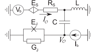
FIG. 2. The proposed quantum synchronization circuit. The resistors Z_{1,2} of Fig. 1 are replaced with a capacitor and an inductor, respectively, forming an oscillator. This results in a big amplification coefficient K \gg 1 close to the resonant frequency \Omega enabling the quantum synchronization. The dc output voltage and current V_O, I_O manifest the quantized transresistance R = V_O/I_O .
