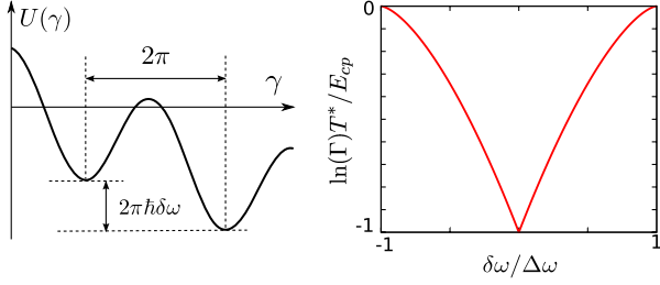
FIG. 4 (color online). Left: Washboard potential for the phase difference \gamma . The hops over the barriers are synchronization errors. Right: The logarithm of the error rate across the synchronization domain.
