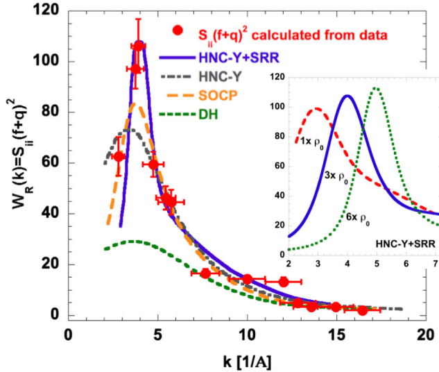
FIG. 3 (color online). Elastic scattering amplitude data measured as a function of scattering vector \mathbf{k} from shock-compressed aluminum for a density of n_e = 5.4 \times 10^{23} \text{ cm}^{-3} and temperature T_e = 10 \text{ eV} . Also shown are various calculations using HNC with quantum potential models of Ref. [10] and the analytical SOCP and DH models of Ref. [26]. Inset: The shift and change in peak intensity of the correlation peak for uncompressed, 3\times , and 6\times compressed aluminum (at T_e = 10 \text{ eV} ), modeled using HNC-Y + SRR, can serve as a density diagnostic.
