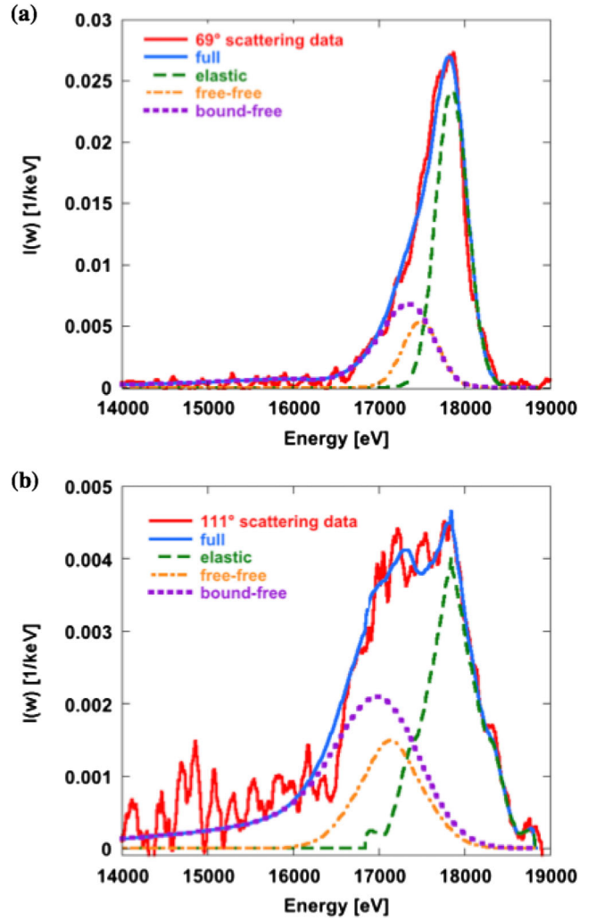
FIG. 2 (color online). Examples of x-ray scattering spectra from singly shocked Al for two different scattering angles. Best fit for the \theta = 69^\circ (a) and 111^\circ (b) experimental data together with the individual contribution from elastic scattering corresponding to the first term in Eq. (3), inelastic scattering from free electrons (free-free scattering) corresponding to the second term in Eq. (3), and inelastic scattering from bound electrons (bound-free scattering) corresponding to the third term in Eq. (3). The full synthetic x-ray scattering spectrum takes into account the sum of these contributions. The experimental spectra have been background corrected and are plotted in absolute units of intensity of the dynamic structure factor.
