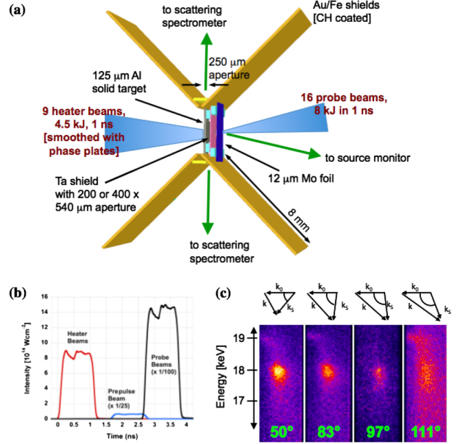
FIG. 1 (color online). (a) Schematic of the experiment showing nine heater beams that compress the Al foil and 16 delayed probe beams that produce E = 17.9 \text{ keV} x rays. X-ray scattering is observed in both the upward and downward directions with gated curved crystal spectrometers. The vertical location of the aperture in the Ta shield defines the two scattering angles on a given shot. (b) Heater, probe, and probe prepulse beam intensities on target. (c) Example of the raw scattering data show that the relative intensity of scattering is broadened and greatly reduced with increasing angle.
