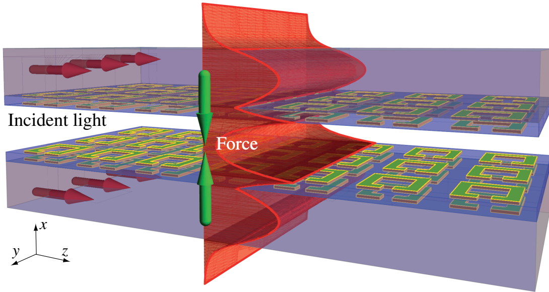
FIG. 1 (color online). The setup to enhance the optical gradient force between two dielectric slab waveguides. A metamaterial cladding indicated by the split-ring resonators is derived from a folding transformation to reduce the distance between the two dielectric waveguides (shown in plain gray) perceived by light. Since the optical gradient force decays with distance, the metamaterial slab allows enhancing the force.
