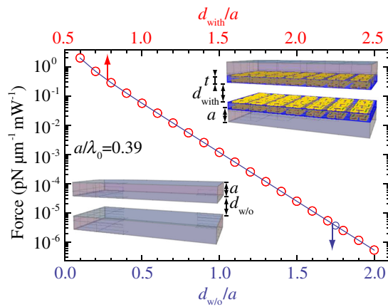
FIG. 2 (color online). Equivalence between the optical force in the traditional configuration of two silicon slab waveguides with n = 3.476 and the transformed setup of silicon waveguides ( n = 3.476 ) with a metamaterial medium attached to it ( n = -1 , t = 0.25a ). The solid blue line shows the optical force between two bare waveguides as a function of the gap distance d_{w/o} . The red circles represent the optical force generated in the transformed configuration as a function of the gap between the metamaterial slabs d_{with} . The metamaterial slab is designed such that d_{with} = d_{w/o} + 0.5a . In these simulations, the fundamental TE modes are considered for a/\lambda_0 = 0.39 , corresponding to a typical setup where \lambda_0 = 1.55 \mu\text{m} and a = 600 \text{ nm} .
