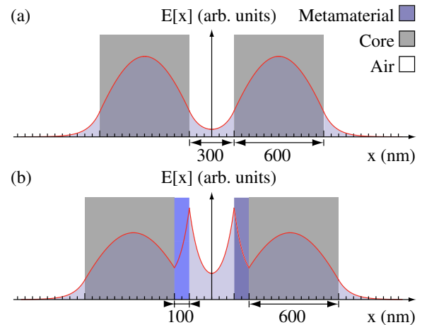
FIG. 3 (color online). Electric field profiles of the fundamental mode in the waveguide pair. (a) The traditional configuration of two slab waveguides indicated by the gray rectangles. If the waveguides are placed close to each other, the evanescent tails interact with the waveguides, resulting in a gradient force between the two slabs. (b) The configuration with a metamaterial cladding as annihilating medium. In between the slab waveguides, we place a metamaterial slab that amplifies the evanescent tails. We demonstrate that this effect enhances the optical gradient force considerably.
