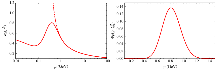
FIG. 1 (color online). Left: Model for the running coupling with freezing in the infrared (solid line) and leading order running coupling with Landau pole (dashed line) for n_f = 3 and \Lambda = 0.25 GeV. Right: Proton impact factor in momentum space with \mathcal{C} = 1/\Gamma(1 + \delta) and \delta, Q_0 with the values used for the comparison to DIS data.
