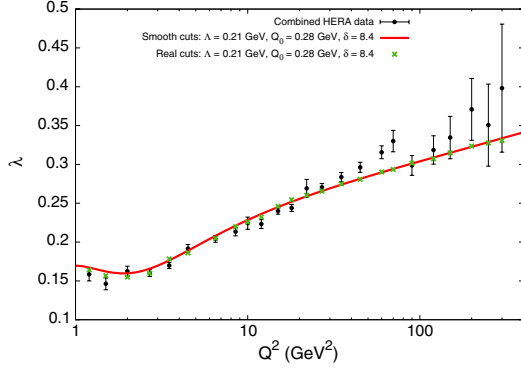
FIG. 2 (color online). Comparison of our prediction with experimental data.
