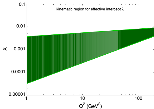
FIG. 3 (color online). Smooth cuts in x used for the effective intercept of F_2 .
