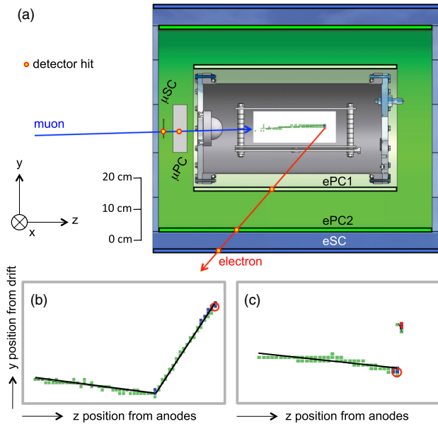
FIG. 1 (color online). Upper panel: (a) Cross-sectional side view of the MuCap detector showing a typical muon stop and decay electron. Lower panels: Zoomed-in special event topologies. (b) Rare large-angle \mu - p scatter event with \sim 10^{-2}/\mu probability. (c) Very rare delayed capture on impurity in \mu O \rightarrow N^* \nu with \sim 3.4 \times 10^{-6}/\mu probability. The interpretation of the event displays is described in the text.
