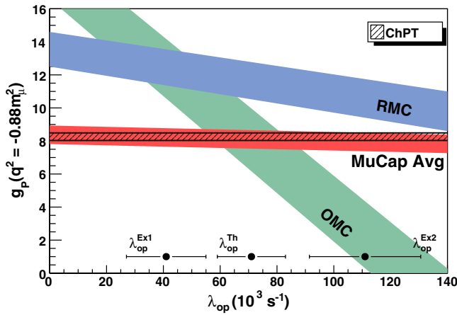
FIG. 2 (color online). Extracted values for g_p as a function of the poorly known molecular transition rate \lambda_{op} [12,13,34]. In contrast to earlier experiments (OMC [11], RMC [14]), MuCap is rather insensitive to this parameter.
