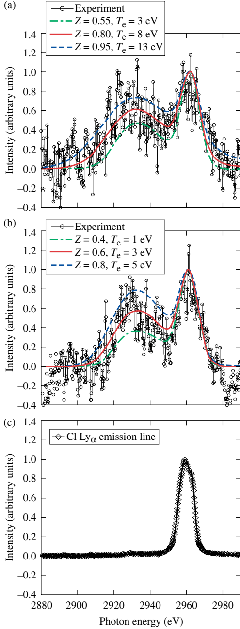
FIG. 3 (color online). Measurement of (a) Cl Ly \alpha emission scattered from shocked liquid deuterium with a 250 \mu\text{m} slit in the scattering channel and simulated scattering spectra, (b) Cl Ly \alpha emission scattered from shocked liquid deuterium without a 250 \mu\text{m} slit in the scattering channel and simulated scattering spectra, (c) Cl Ly \alpha emission incident on the shocked liquid deuterium. The inferred plasma conditions in (a) are T_e = 8 \pm 5 \text{ eV} , Z \sim 0.8(-0.25, +0.15) , and n_e = 2.2(\pm 0.5) \times 10^{23} \text{ cm}^{-3} , and in (b) are T_e = 3 \pm 2 \text{ eV} , Z \sim 0.6 \pm 0.2 , and n_e = 2.0(\pm 0.5) \times 10^{23} \text{ cm}^{-3} .
