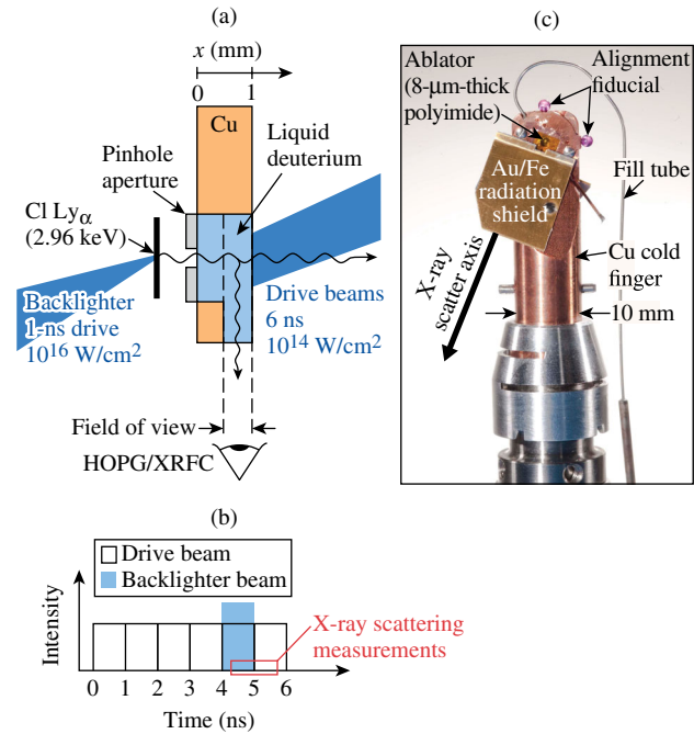
FIG. 1 (color online). (a) Schematic of the x-ray Thomson scattering experiment. An 8- \mu\text{m} CH ablator was irradiated with a constant-intensity, 6-ns UV laser drive, launching a shock wave through a cryogenic cell filled with liquid deuterium and creating warm, dense matter. Sixteen tightly focused beams irradiated a parylene D backlighter at 10^{16} \text{ W/cm}^2 , producing CI Ly \alpha emission that was scattered at \sim 90^\circ and detected with an x-ray framing camera outfitted with a HOPG crystal spectrometer. (b) Timing of the drive and backlighter beams and the x-ray scattering measurements. (c) Photograph of the cryogenic x-ray Thomson scattering target. The fill tube directs deuterium gas into the cryogenic cell, where it condenses into liquid. The ruby tooling balls on the top and right sides of the Cu cold finger are target alignment fiducials. The Au/Fe shield blocks a direct line of sight between the laser-produced plasmas and the detector, which is positioned \sim 90^\circ to the laser drive axis.
