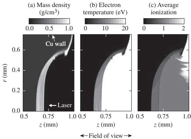
FIG. 2. Contour plots of (a) mass density, (b) electron temperature, and (c) average ionization of shocked liquid deuterium at 5 ns, predicted using DRACO.
