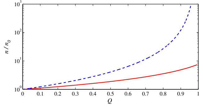
FIG. 1 (color online). Optimized density profiles for (a) the axial density gradient method (dashed line), with Q = z/L signifying an axially inhomogeneous density profile, and (b) the perpendicular magnetic compression method (solid line), with Q = t/T signifying a time-varying, but axially uniform, density profile. Note that L = cT .
