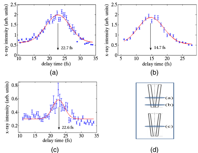
FIG. 4 (color online). The cross-correlation data (blue dots) measured at different double-slot arrays, as shown in (d). For (a) and (b), the beam was on the wide-slot area with a different slot separation. For (c), the slot separation is same as that in (a), but the slot width is narrower. Gaussian fitting results are shown with red curves.
