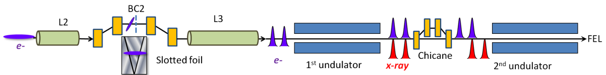
FIG. 1 (color online). A schematic layout of the emittance spoiling foil and cross-correlation configuration at the LCLS. A double-slotted foil setup is used for the illustration in this figure.
