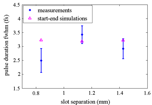
FIG. 6 (color online). The measured pulse duration vs slot separation with a same condition in Fig. 5. Triangles show the start-to-end simulation results.
