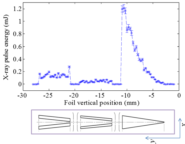
FIG. 2 (color online). Measured FEL pulse energy (blue stars) vs foil vertical position. A motor controls the foil vertical position to have electrons pass through different slot arrays (bottom).
