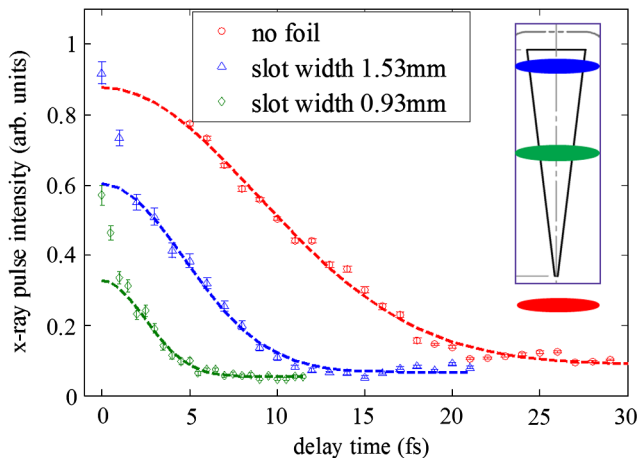
FIG. 3 (color online). Cross-correlation measurements for a single bunch: no foil (red circles), with slot width 1.53 mm (blue triangles) and with slot width 0.93 mm (green diamonds). The dashed lines show Gaussian fit results (fitting is from a minimum delay of 2 fs). With a deconvolution factor 1.5, the obtained FWHM x-ray pulse durations are 14.1, 7.3, and 3.8 fs.
