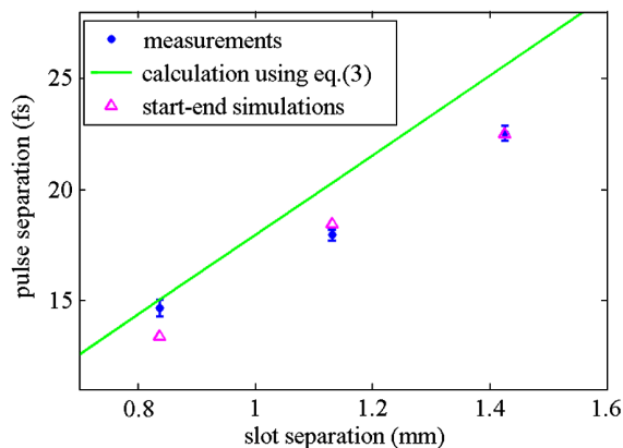
FIG. 5 (color online). The measured pulse delay vs slot separation (blue dots) at 8.3 keV photon energy, using the wide double-slot area. The calculation result using Eq. (3) is shown in a solid green line. Start-to-end simulation results are shown with triangles.
