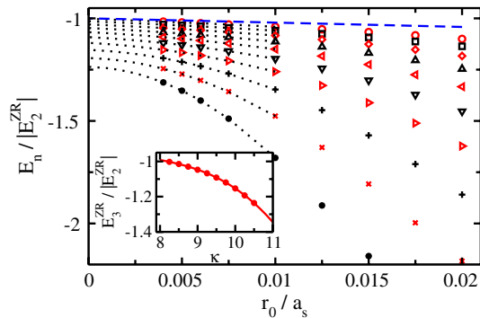
FIG. 1 (color online). Scaled energies as a function of r_0/a_s . The dashed line shows E_2/|E_2^{\text{ZR}}| . The symbols show E_3/|E_2^{\text{ZR}}| for \kappa = 8.25 – 10.5 (top to bottom), in steps of 0.25 ; E_3 is determined by the stochastic variational approach. Dotted lines show three-parameter fits. Inset: Symbols show E_3^{\text{ZR}}/|E_2^{\text{ZR}}| as a function of \kappa . The solid line shows a four-parameter fit.
