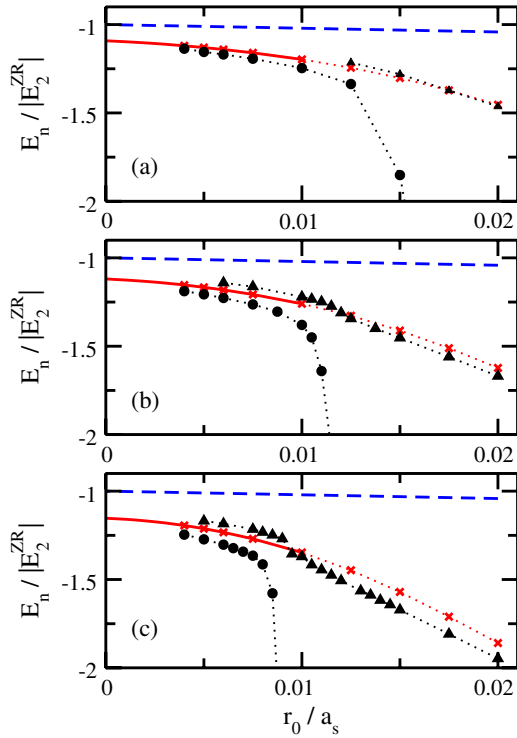
FIG. 2 (color online). Scaled energies as a function of r_0/a_s for (a) \kappa = 9.5 , (b) \kappa = 9.75 , and (c) \kappa = 10 . The dashed lines show E_2/|E_2^{ZR}| , while the crosses (stochastic variational energies) and solid lines (fit) show E_3/|E_2^{ZR}| (these energies are also shown in Fig. 1). Circles and triangles show E_4/|E_2^{ZR}| for the energetically lowest-lying and second-lowest-lying four-body states, respectively. Dotted lines serve as a guide to the eye.
