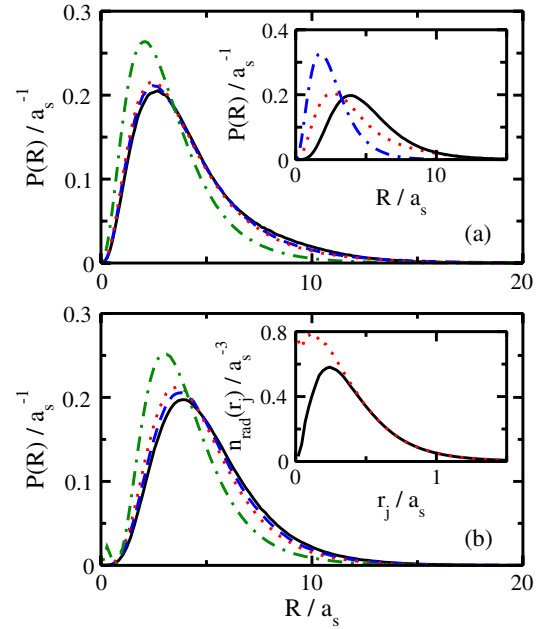
FIG. 3 (color online). (a) Solid, dashed, dotted, and dash-dotted lines show P(R) of the energetically lowest-lying state for n = 3 , \kappa = 8.5 , and r_0/a_s = 0.004, 0.005, 0.006 , and 0.015 , respectively. Inset: Dotted, dash-dotted, and solid lines show P(R) for n = 3 ( \kappa = 8.5 and r_0/a_s = 0.004 ), n = 3 ( \kappa = 9.75 and r_0/a_s = 0.004 ), and n = 4 ( \kappa = 9.75 and r_0/a_s = 0.004 ), respectively. (b) Solid, dashed, dotted, and dash-dotted lines show P(R) for n = 4 , \kappa = 9.75 , and r_0/a_s = 0.004, 0.005, 0.006 , and 0.015 , respectively. For r_0/a_s = 0.004, 0.005 , and 0.006 , the energetically lowest-lying state is considered. For r_0/a_s = 0.015 , the energetically second-lowest-lying state is considered. Inset: Solid and dotted lines show n_{\text{rad}}(r_j) for the heavy and light particles, respectively, for n = 4 , \kappa = 9.75 , r_0/a_s = 0.004 , and 1^+ symmetry.
