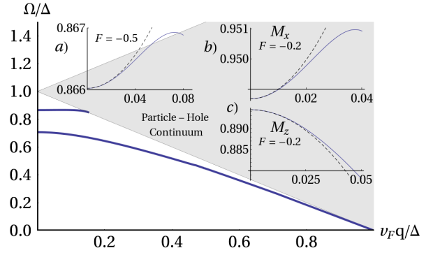
FIG. 2 (color online). Spectrum of chiral spin waves for F_0^a = -0.5 . Inset (a): zoom of the small- q region for the x mode. Insets (b) and (c): spectra of the x and z modes, respectively, for F_0^a = -0.2 and small values of q . The dashed curves represent the parabolic approximation.
