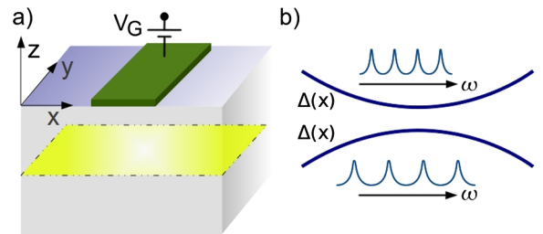
FIG. 3 (color online). (a) Sketch of the suggested experimental setup. Top gate modulates the SO splitting. (b) Top: A minimum in \Delta confines the x mode with a positive effective mass. Bottom: A maximum in \Delta confines the z mode. The corresponding microwave absorption spectra are shown schematically.
