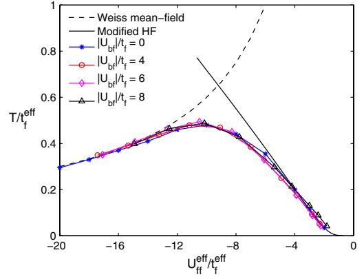
FIG. 3 (color online). The phase diagrams of Fig. 2 can be collapsed onto the phase diagram of a pure fermionic model with renormalized hoppings t_f^{\text{eff}} = t_f - c_2' U_{bf}^2 / U_{bb} and on site repulsions U_{ff}^{\text{eff}} = U_{ff} - c_1' U_{bf}^2 / U_{bb} , with c_1' and c_2' fitting constants. Error bars are of the order of the symbol size and omitted for clarity.
