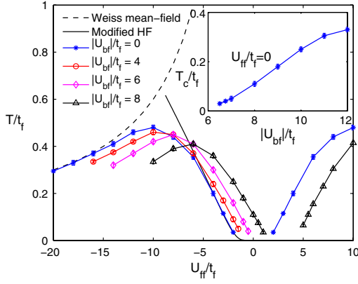
FIG. 2 (color online). S -wave superfluid (left) and antiferromagnetic ( U_{bf} = 0 and |U_{bf}|/t_f = 8 on the right) phase transition of the Bose-Fermi Hubbard model on the 3d cubic lattice at filling n_b = 1 and n_f = n_l = 1/2 and with U_{bb}/t_f = 20 and t_b/t_f = 1 for different boson-fermion interactions U_{bf} . The DMFT results interpolate between the Weiss mean-field result and the T -matrix or BCS result (“modified HF”) (see text). Inset: Critical temperature for pairing for noninteracting fermions ( U_{ff} = 0 ) as a function of the boson-fermion interaction U_{bf} . The transition temperature is exponentially suppressed at low U_{ff} for all U_{bf} (not shown).
