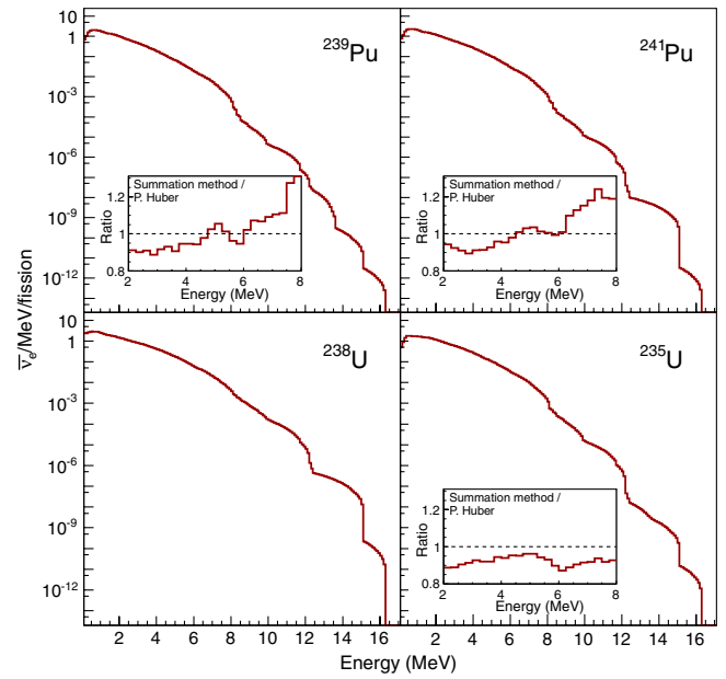
FIG. 1 (color online). Reconstructed antineutrino energy spectra, including the latest TAS data from Ref. [10]. In the insets are the ratios of the spectra to the ones computed by Huber [19].
