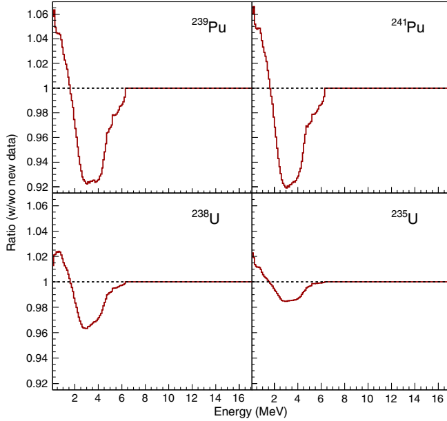
FIG. 2 (color online). Ratios between two spectra built with the data set described in the text over the same but the new TAS data.
