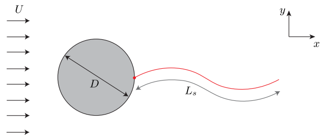
FIG. 1 (color online). The simply supported elastic filament anchored to a rigid cylinder subject to a uniform streamwise flow. The initial configuration is symmetric with respect to the normal coordinate y , which is centered on the cylinder.
