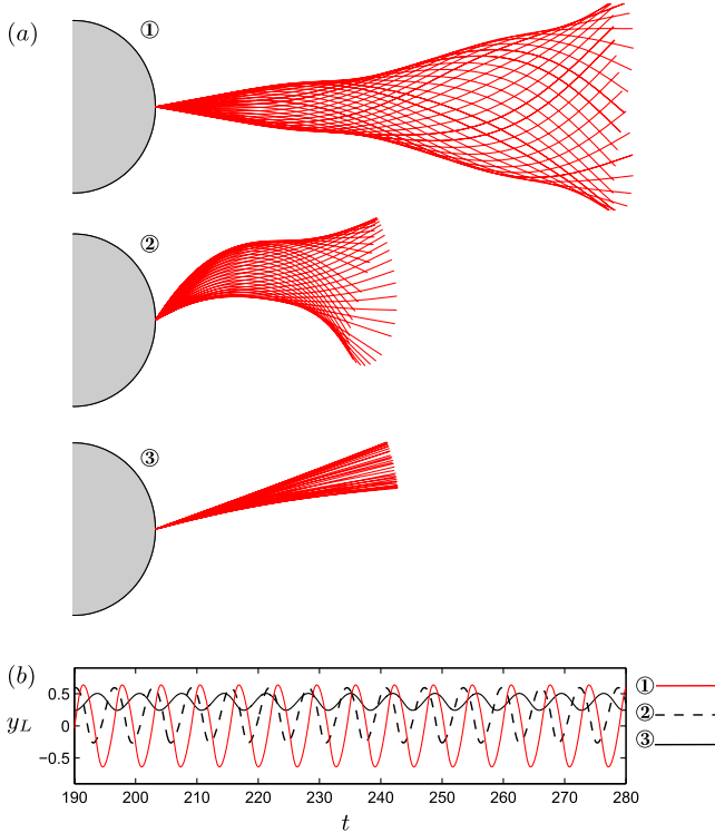
FIG. 2 (color online). Solid (red) lines in (a) depict the filament position at different times. The symmetric flapping filament ( L = 3 , R_2 = 0.005 ) is marked with label ①, whereas asymmetric flapping filaments, corresponding to a flexible ( L = 1.5 , R_2 = 0.005 ) or rigid ( L = 1.5 , R_2 = 0.1 ) configuration, are marked with labels ② and ③, respectively. For all cases, the other parameters are fixed at \text{Re} = 100 and R_1 = 0.1 . In (b), the transverse component of the filament tail position y_L is shown as a function of time.
