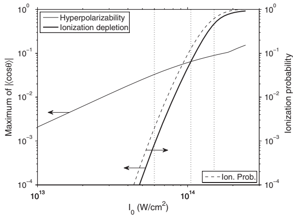
FIG. 3. Solid curves: The maximum field-free orientation ( |\langle \cos\theta \rangle| ) for the two mechanisms, as a function of pump intensity. Each of the two colors in the pump pulse has intensity I_0 . The thin curve is for the hyperpolarizability mechanism; thick curve is for the ionization depletion. Dashed curve: Total ionization probability that occurs during the ionization depletion mechanism. Vertical lines: The vertical dotted lines mark the intensities used in Figs. 4 and 5.
