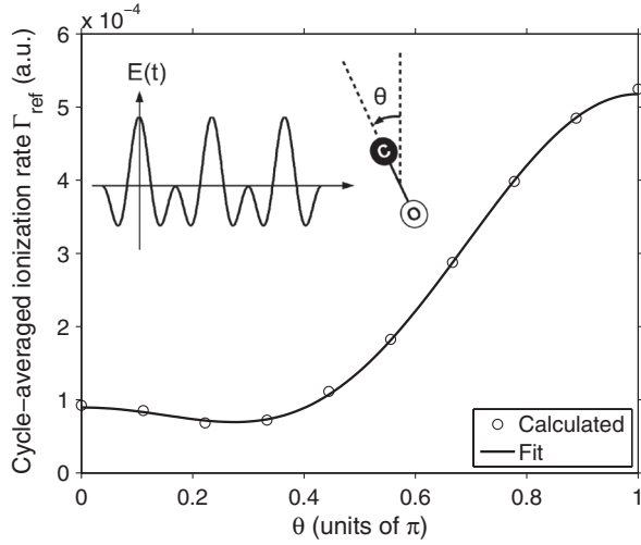
FIG. 2. Cycle-averaged ionization rate \Gamma_{\text{ref}}(\theta) . Shown are the numerically calculated rates, and the fit from Eq. (8). Inset depicts the angle \theta . For \theta = 0^\circ , the molecule is oriented such that the largest electric field oscillation of the two-color field points from O to C.
