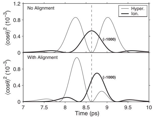
FIG. 6. Orientation revivals within the impulsive approximation ( I_0 = 6.0 \times 10^{13} W/cm 2 ). The ionization depletion results are scaled by a factor of 1000. Top panel: revival structure with the alignment interaction turned off ( \lambda_P = 0 ). Bottom panel: with the alignment interaction included. The vertical dashed line denotes the revival time t_{\text{rev}} .
