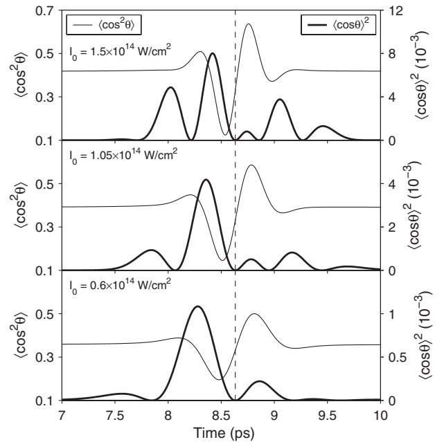
FIG. 4. The hyperpolarizability orientation mechanism. Alignment (thin line, left axis) and orientation (thick line, right axis) wave-packet revivals for a selection of intensities. The vertical dashed line denotes the revival time t_{\text{rev}} .
