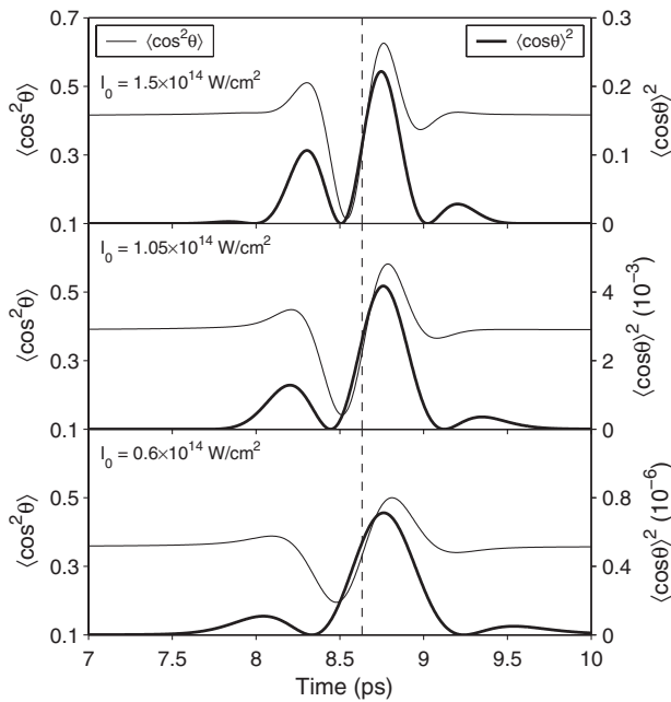
FIG. 5. The ionization depletion mechanism. See Fig. 4.
