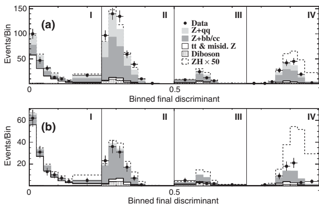
FIG. 1. Distribution of the BFD output for all candidates meeting Tx or LL (a) and TT or TL (b) selections, compared to the sum of the expectation from background. A variable bin width is used to maintain sufficient statistics in simulated samples. The labels (I, II, III, IV) and vertical solid lines indicate the regions defined by the multistage discriminant method.
