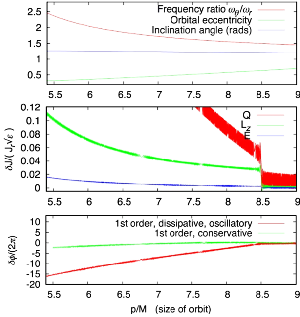
FIG. 1 (color online). [Top] The adiabatic inspiral computed from our approximate post-Newtonian self-force, for a mass ratio \varepsilon = \mu/M = 3 \times 10^{-6} , with black hole spin parameter a = 0.95 , with initial conditions semilatus rectum p = 9.0M , eccentricity e = 0.7 , and orbital inclination \theta_{\text{inc}} = 1.20 . The bottom curve is e , the middle curve is \theta_{\text{inc}} , and the top curve is ratio of frequencies \omega_\theta/\omega_r , shown as functions of p . [Middle] The fluctuating, dissipative part of the first-order self-force causes a strong resonance when \omega_\theta/\omega_r = 3/2 at p = 8.495 . Shown are the corrections to the energy E , angular momentum L_z and Carter constant Q , as functions of p , scaled to their values at resonance and divided by the square root \sqrt{\mu/M} of the mass ratio. The sudden jumps at the resonance are apparent, with the largest occurring for the Carter constant. [Bottom] The lower curve is the correction to the number of cycles \phi/(2\pi) of azimuthal phase of the inspiral caused by the fluctuating, dissipative part of the first order self-force. The sharp downward kick due to the resonance at p = 8.495 can be clearly seen. The resonant corrections to the number of cycles of r and \theta motion are similar. These phase shifts scale as \sqrt{M/\mu} . The upper curve is the postadiabatic phase correction due to the conservative piece of the first order self-force, which is considerably smaller and is independent of the mass ratio.
