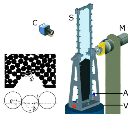
FIG. 1 (color online). Sketch of the experimental setup. Key: C, video camera; A, accelerometer; V, electromagnetic shaker; M, motor; S, silo. On the left, a photograph of an arch is presented, indicating the angle \phi for one bead. We also show a diagram of a horizontal defect as considered in the text. Forces for the right side of the bead are represented with dashed vectors, from left to right: weight, normal force, and friction.
