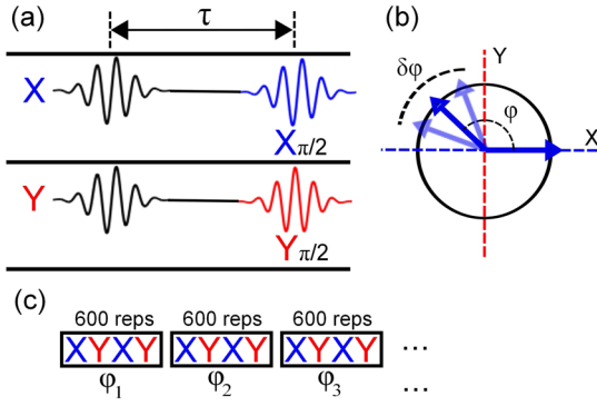
FIG. 2 (color online). The Ramsey tomography oscilloscope protocol. (a) Four Ramsey sequences are performed: two with the final \pi/2 pulse about the \pm X axes and two with the final \pi/2 pulse about the \pm Y axes. The precession time for both sequences is fixed at \tau = 100 ns. (b) The combined X axis and Y axis sequences constitute tomography of the state in the x, y plane after precession by \tau , thereby measuring the angle \varphi traversed by the state. (c) Several hundred subsequent X and Y measurements are grouped together to get an average value for \varphi . The entire process is repeated once per second for several hours to build up a time series \delta f(t) = \delta \varphi(t)/2\pi\tau .
