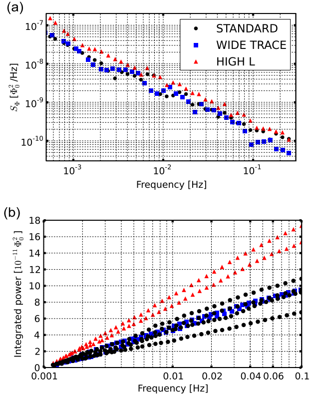
FIG. 3 (color online). Power spectra for each inductor design. (a) Typical spectra for each type of device. (b) Spectral power integrated over the range 0.001 to 0.1 Hz. In (a) we plot only one spectrum for each device design for clarity in the plot. In (b) we show several curves, measured at several bias points, in devices all fabricated on the same wafer.
