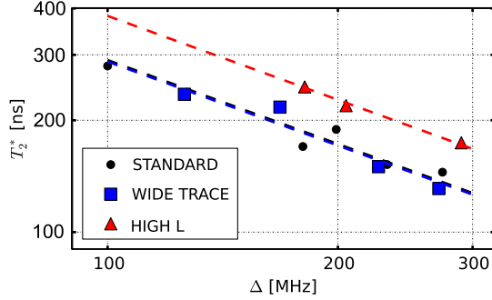
FIG. 4 (color online). Plot of Ramsey decay time T_2^* vs non-linearity \Delta for each type of device. Each point comes from a fit to Eq. (3). For each bias flux, T_1 and \Delta are measured in separate experiments. Dashed fit lines are drawn with the predicted slope of -3/4 in order to compare magnitudes. The fit lines for the standard and wide trace designs fall on top of one another. The high inductance devices show an increase in T_2^* by a factor of 1.3. Confidence bounds, typically 2% of data values, cannot be seen on this scale.
