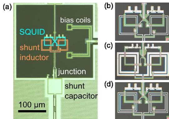
FIG. 1 (color online). Phase qubit devices used in the experiments. Panel (a) shows the readout SQUID, inductor coils, bias coils, and shunt capacitor; panels (b), (c), and (d) show close-ups of the inductors and SQUIDs. Panel (b) shows the standard qubit coils, (c) the wide trace coils, and (d) the high inductance coils. Horizontal image lengths are (b) 117 \mu\text{m} , (c) 173 \mu\text{m} , and (d) 123 \mu\text{m} . Device parameters are given in Table I.
